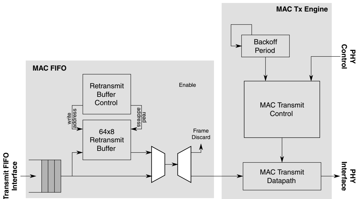
Figure 44-57. Packet Re-Transmit Overview
