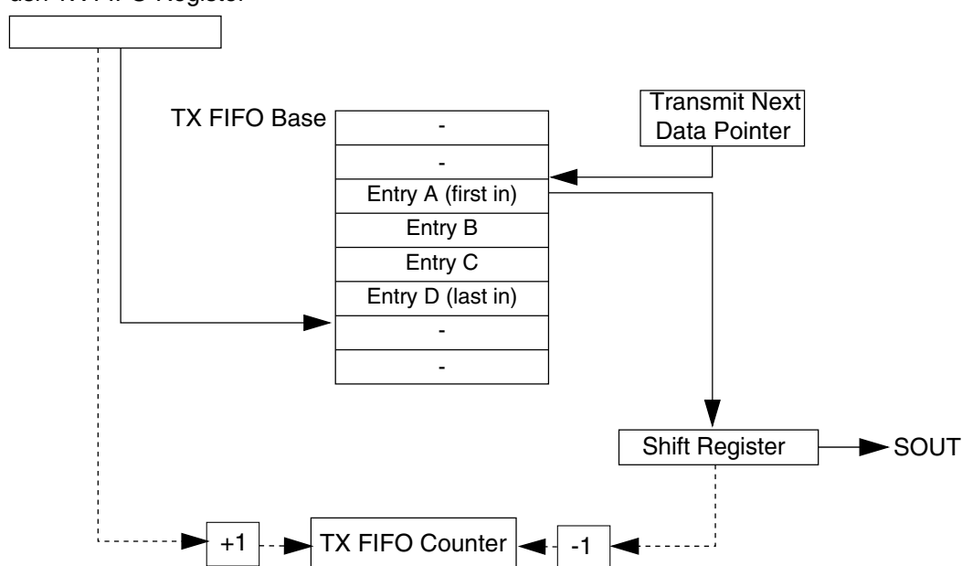
Figure 49-100. TX FIFO Pointers and Counter
