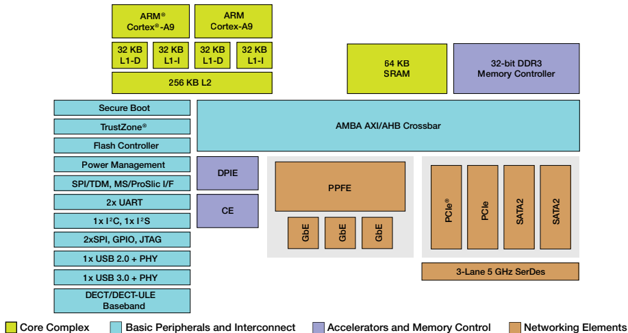
QorIQ LS1024A Communications Processor Block Diagram
