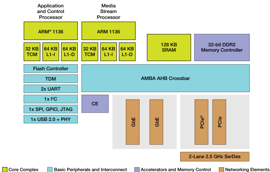
QorIQ LS102MA Communications Processor Block Diagram
