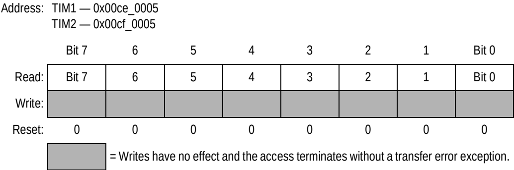
Figure 15-7. Timer Counter Register Low (TIMCNTL)
