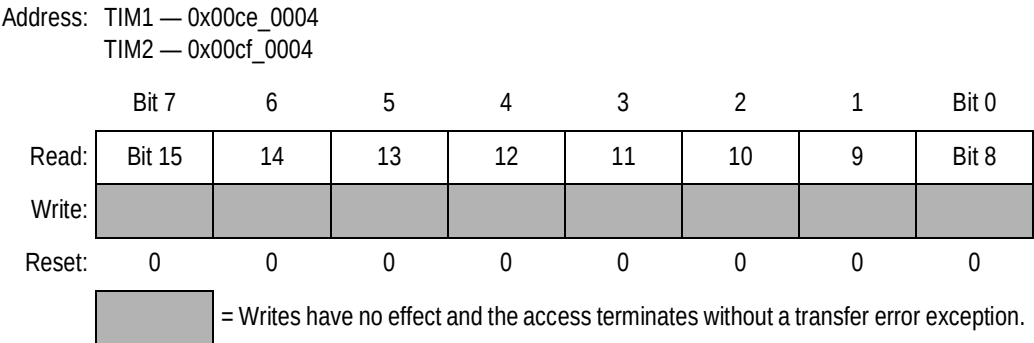
Figure 15-6. Timer Counter Register High (TIMCNTH)
