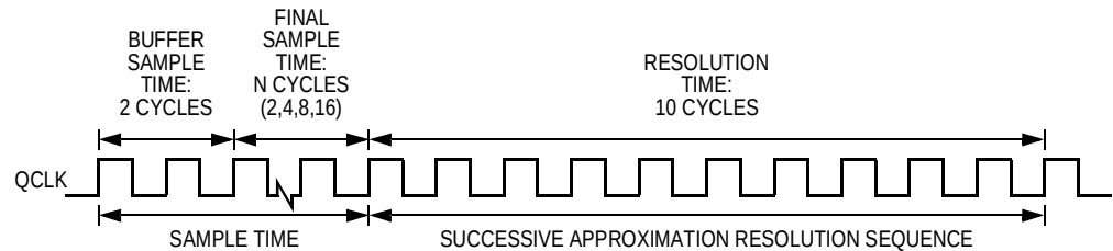
Figure 18-20. Conversion Timing
