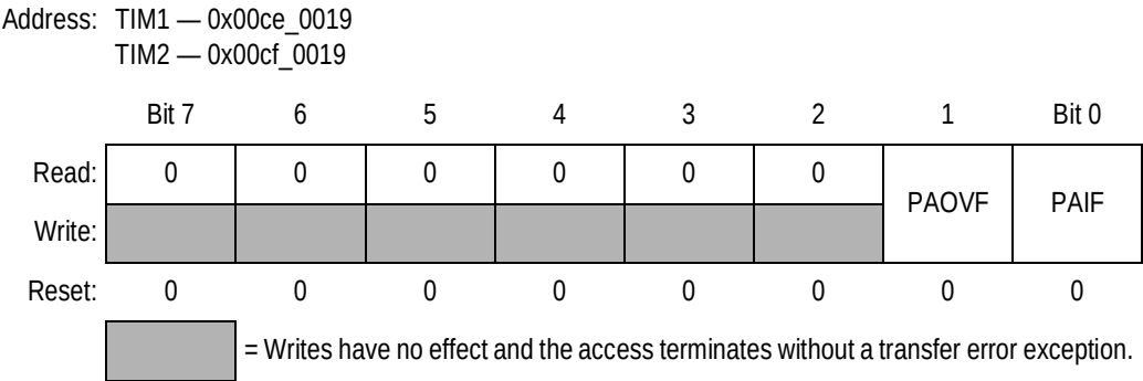
Figure 15-20. Pulse Accumulator Flag Register (TIMPAFLG)
