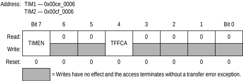
Figure 15-8. Timer System Control Register (TIMSCR1)
