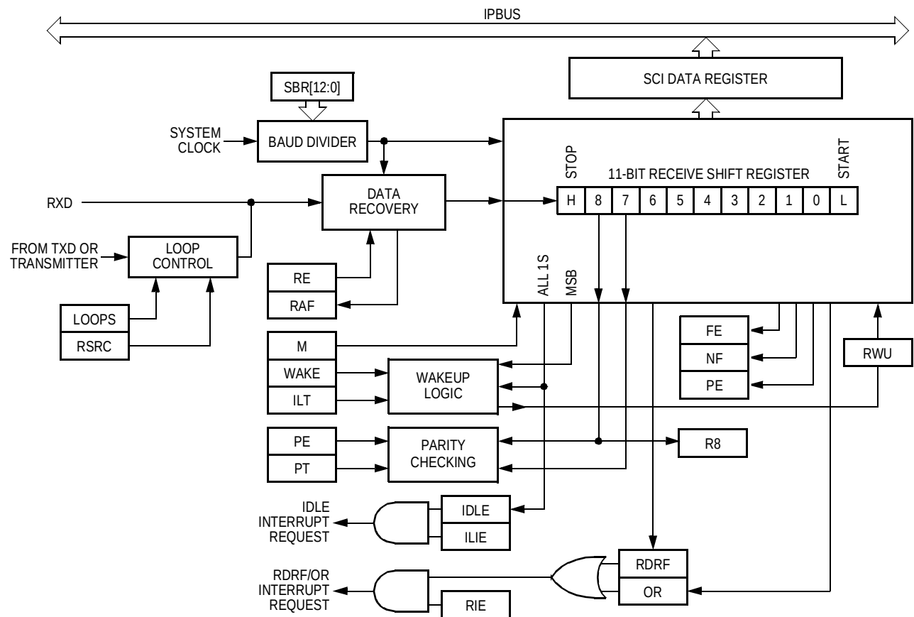
Figure 16-15. SCI Receiver Block Diagram
