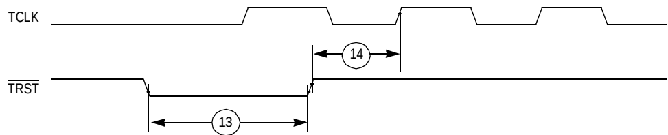
Figure 22-12. TRST Timing
