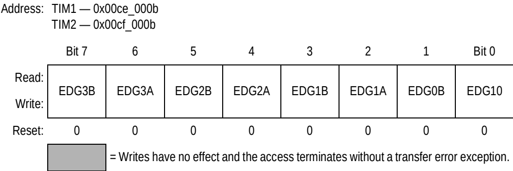
Figure 15-12. Timer Control Register 2 (TIMCTL2)
