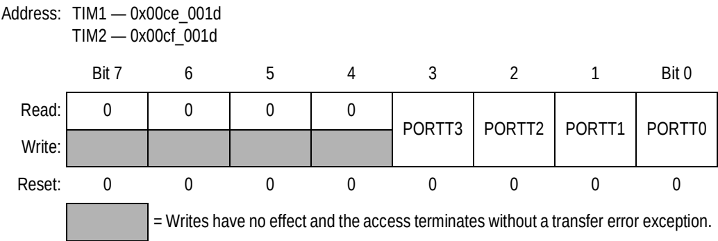
Figure 15-23. Timer Port Data Register (TIMPORT)
