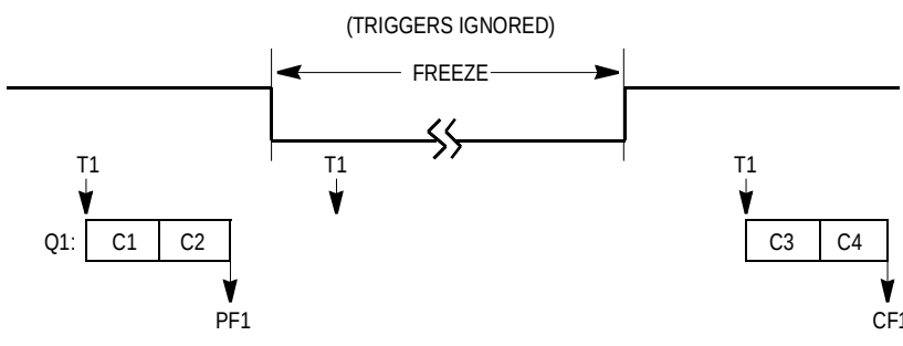
Figure 18-38. CCW Freeze Situation 16
