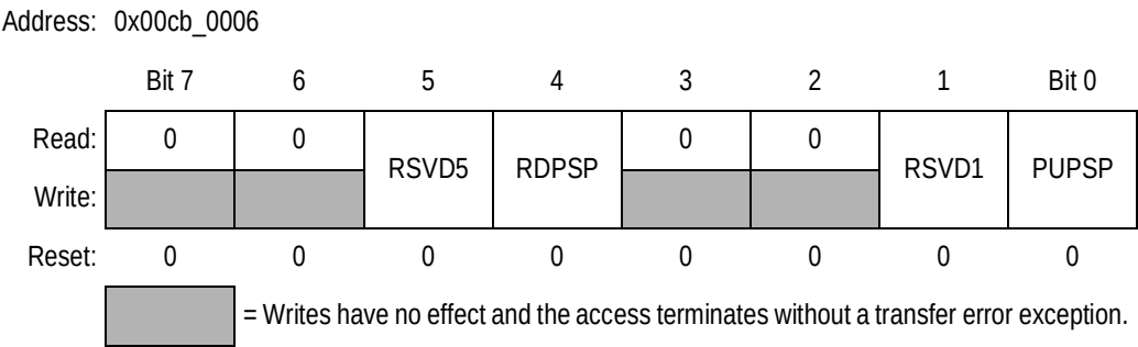
Figure 17-7. SPI Pullup and Reduced Drive Register (SPIPURD)
