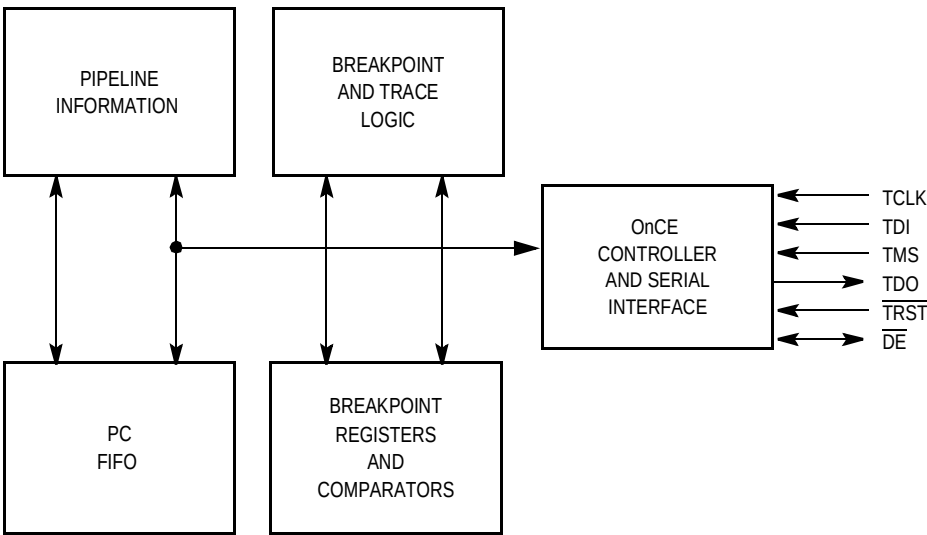
Figure 21-4. OnCE Block Diagram
