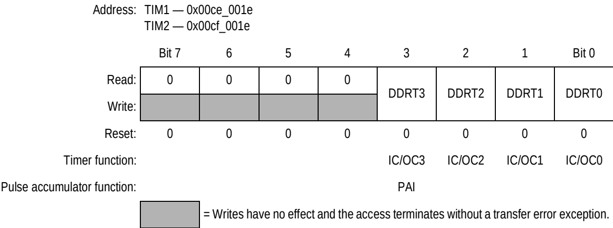
Figure 15-24. Timer Port Data Direction Register (TIMDDR)
