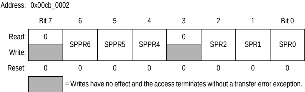
Figure 17-4. SPI Baud Rate Register (SPIBR)
