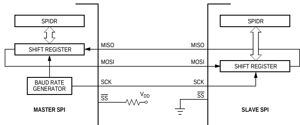
Figure 17-10. Full-Duplex Operation
