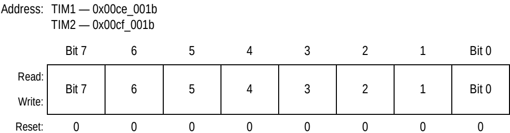
Figure 15-22. Pulse Accumulator Counter Register Low (TIMPACNTL)
