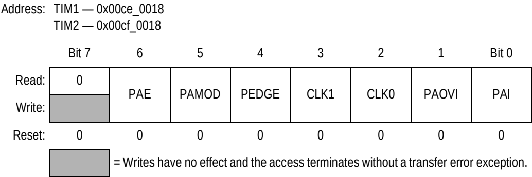
Figure 15-19. Pulse Accumulator Control Register (TIMPACTL)
