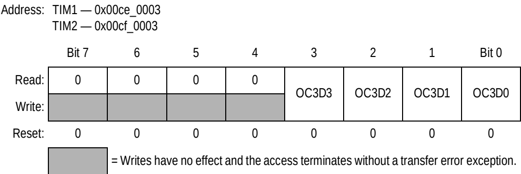
Figure 15-5. Timer Output Compare 3 Data Register (TIMOC3D)
