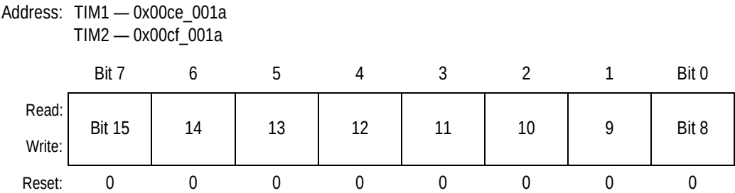
Figure 15-21. Pulse Accumulator Counter Register High (TIMPACNTH)
