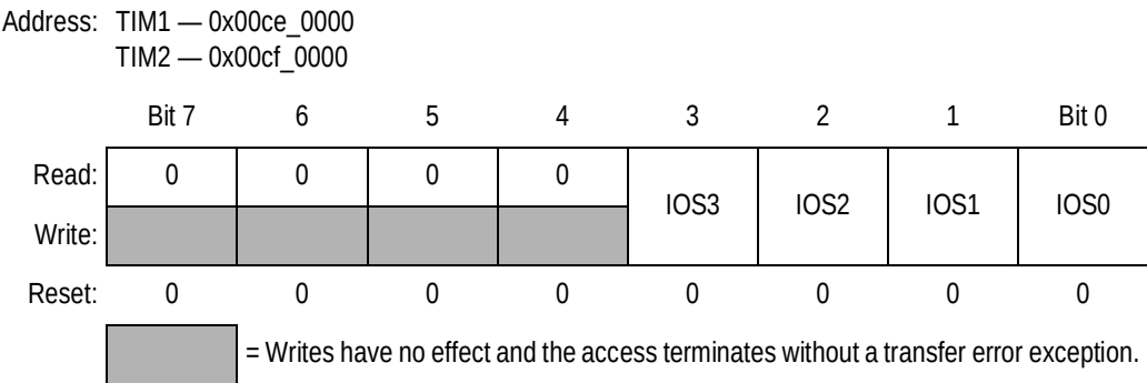
Figure 15-2. Timer Input Capture/Output Compare Select Register (TIMIOS)
