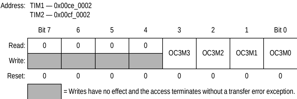
Figure 15-4. Timer Output Compare 3 Mask Register (TIMOC3M)
