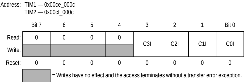
Figure 15-13. Timer Interrupt Enable Register (TIMIE)
