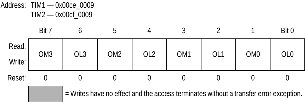
Figure 15-11. Timer Control Register 1 (TIMCTL1)
