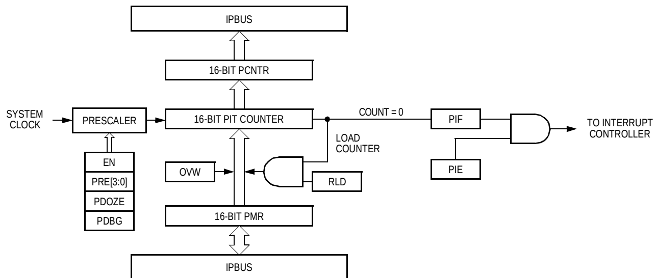
Figure 14-1. PIT Block Diagram
