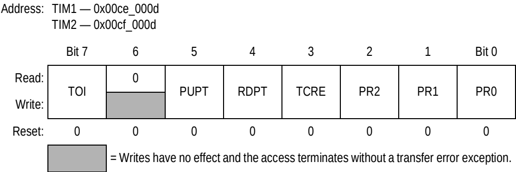
Figure 15-14. Timer System Control Register 2 (TIMSCR2)
