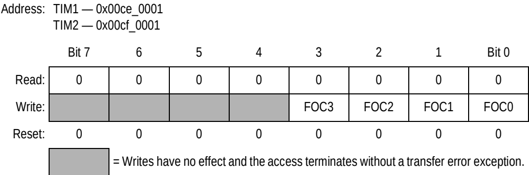
Figure 15-3. Timer Compare Force Register (TIMCFORC)
