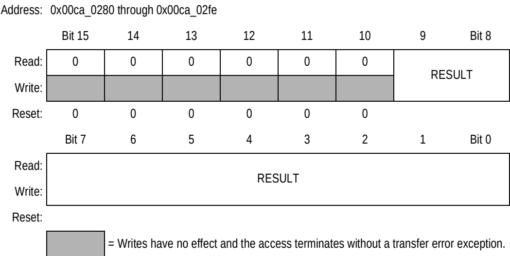
Figure 18-15. Right-Justified Unsigned Result Register (RJURR)
