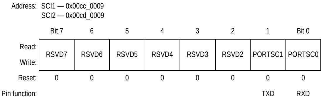
Figure 16-11. SCI Port Data Register (SCIPORT)
