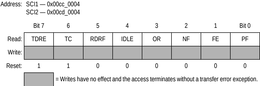
Figure 16-6. SCI Status Register 1 (SCISR1)
