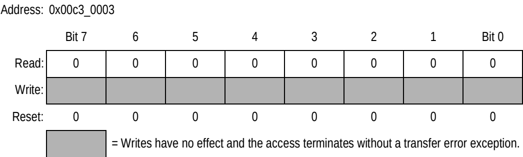
Figure 10-4. Synthesizer Test Register (SYNTR)
