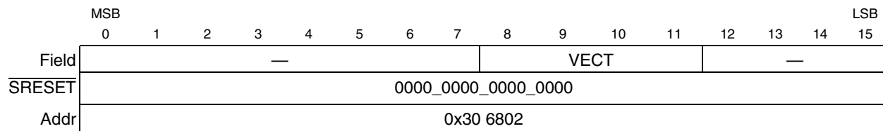
Figure 17-5. Vector Register (MIOS14VECT)
