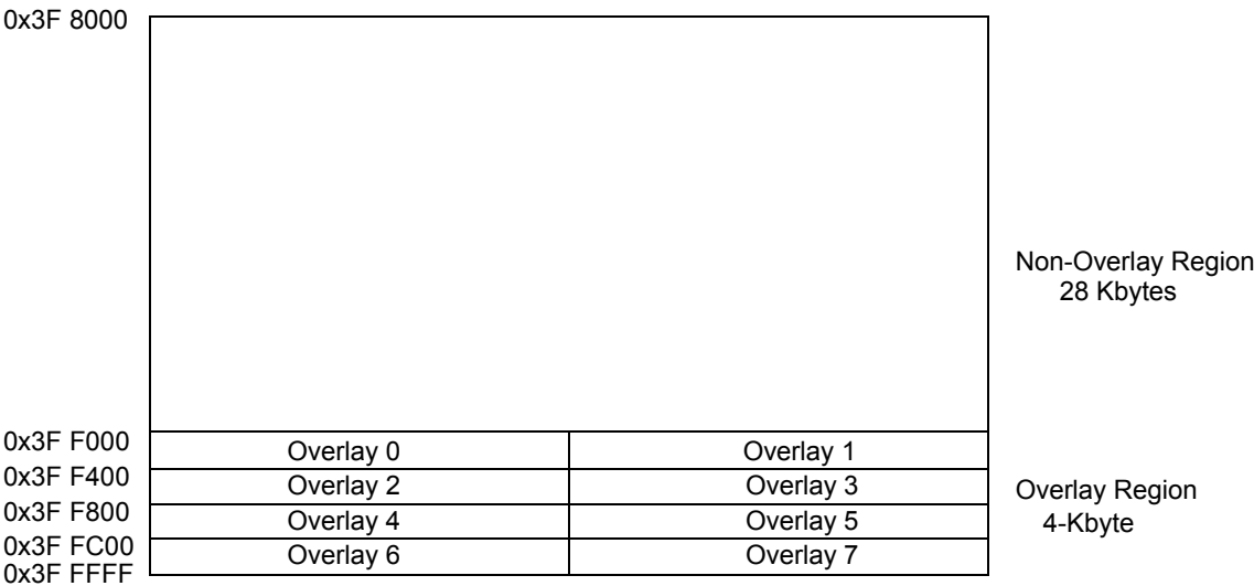
Figure 22-4. CALRAM Array
