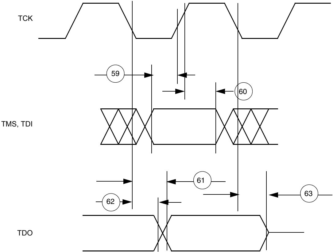
Figure G-37. JTAG Test Access Port Timing Diagram
