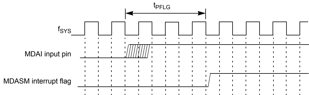
Figure F-59. MDASM Input Pin to MDASM Interrupt Flag Timing Diagram
