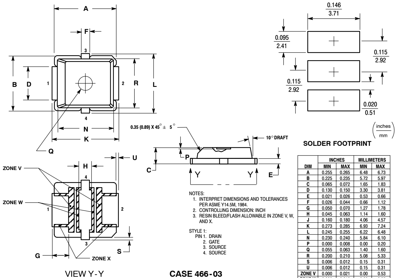
CASE 466-03 ISSUE D PLD-1.5 PLASTIC
