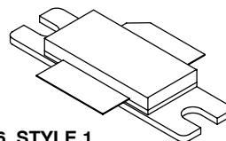
CASE 465-06, STYLE 1 NI-780 MRF18085ALR3
