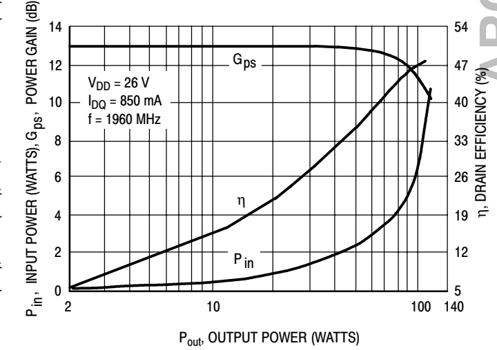
Figure 8. CW Performance
