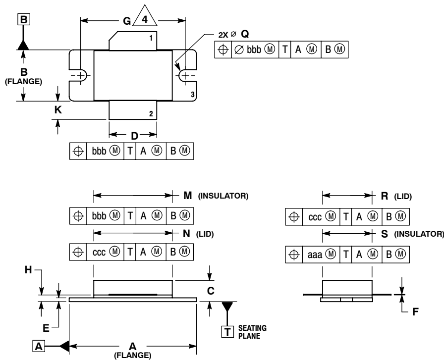
CASE 465B-03 ISSUE D NI-880 MRF6S23140HR3
