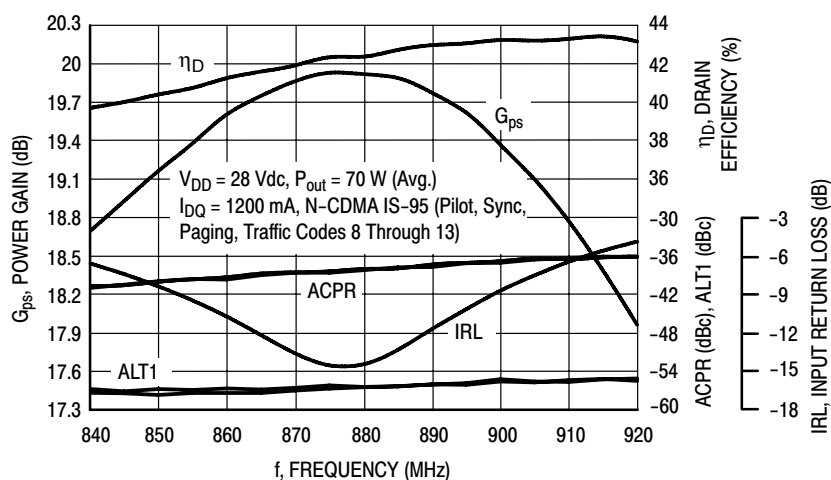
Figure 4. Single-Carrier N-CDMA Broadband Performance @ P out = 70 Watts Avg.
