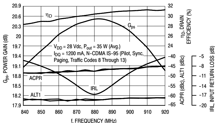
Figure 3. Single-Carrier N-CDMA Broadband Performance @ P out = 35 Watts Avg.
