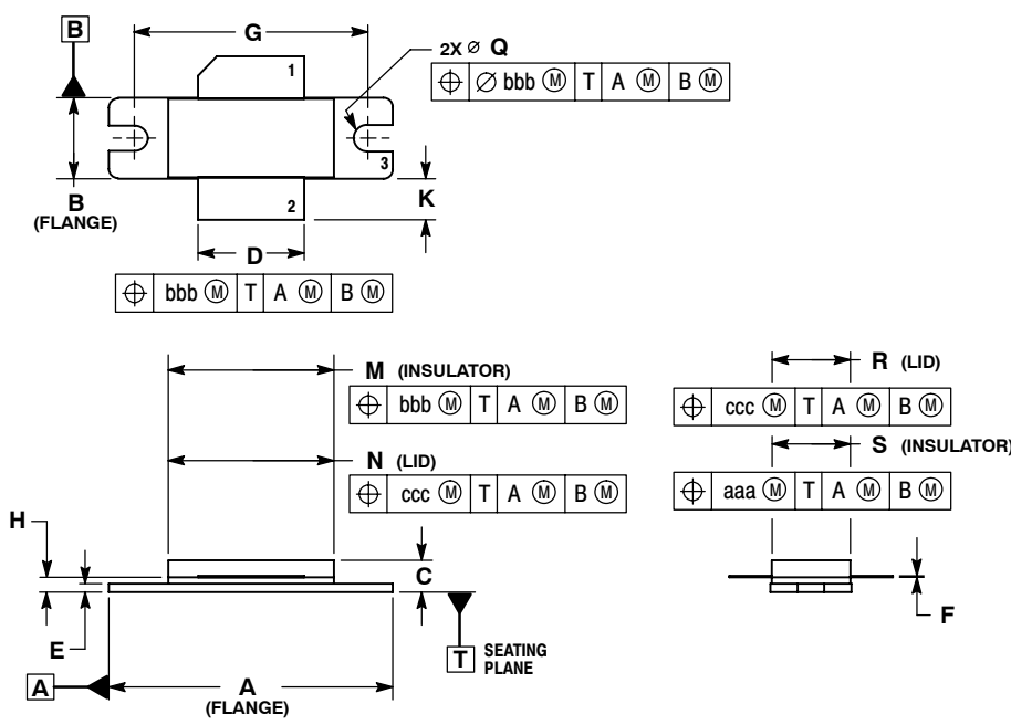
CASE 465-06 ISSUE G NI-780 MRFE6S9201HR3
