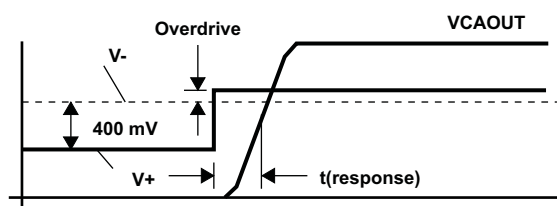
Figure 5-9. Overdrive Definition
