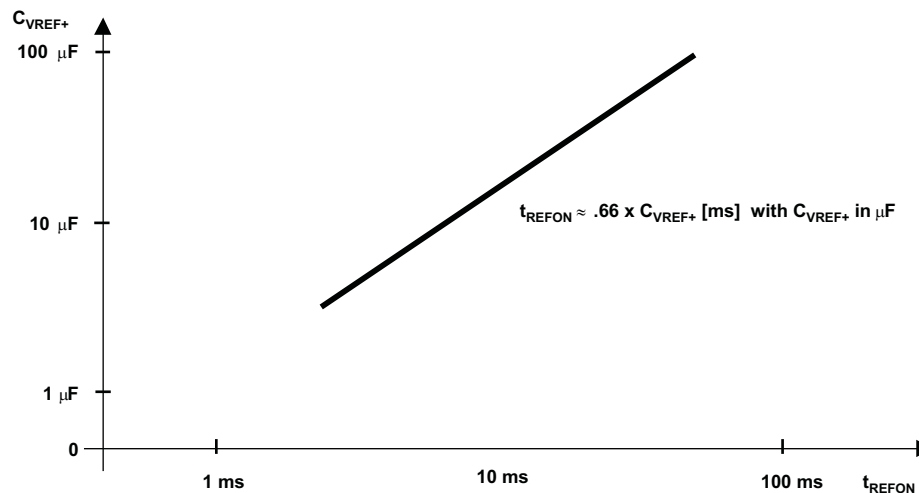
Figure 5-18. Typical Settling Time of Internal Reference t_{REFON} vs External Capacitor on V REF+
