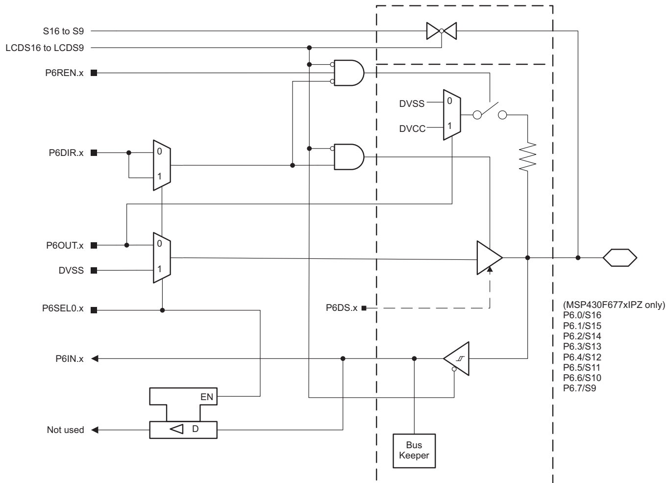
Figure 6-26. Port P6 (P6.0 to P6.7) Diagram (MSP430F677xIPZ Only)
