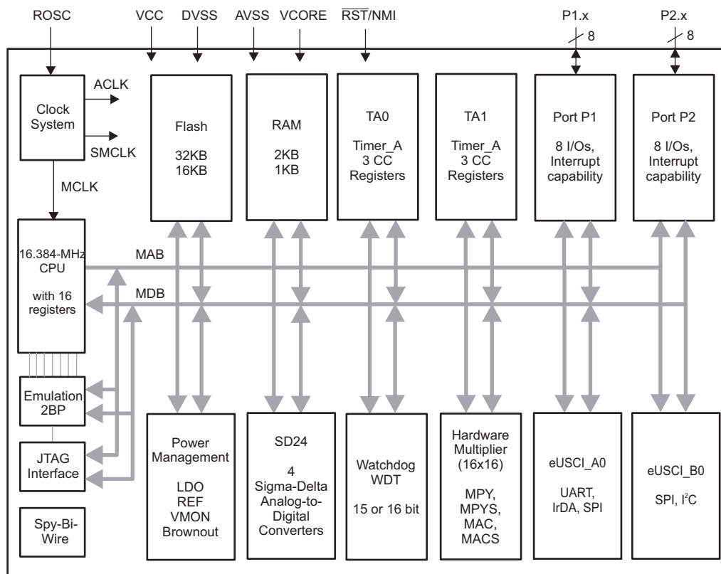
Figure 6-1. Functional Block Diagram – RHB Package – MSP430i2041, MSP430i2040
