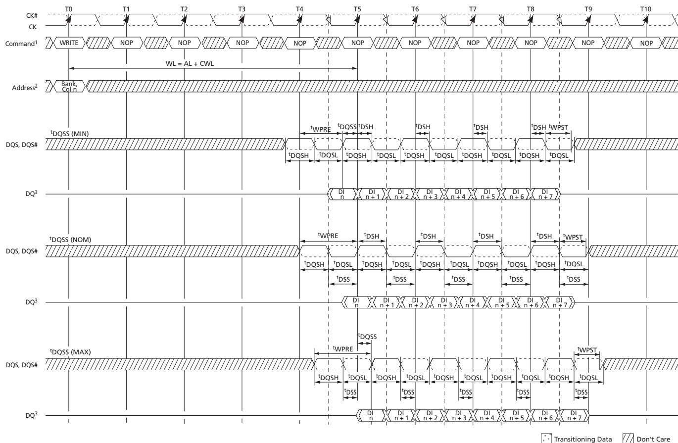
Figure 82: WRITE Burst
