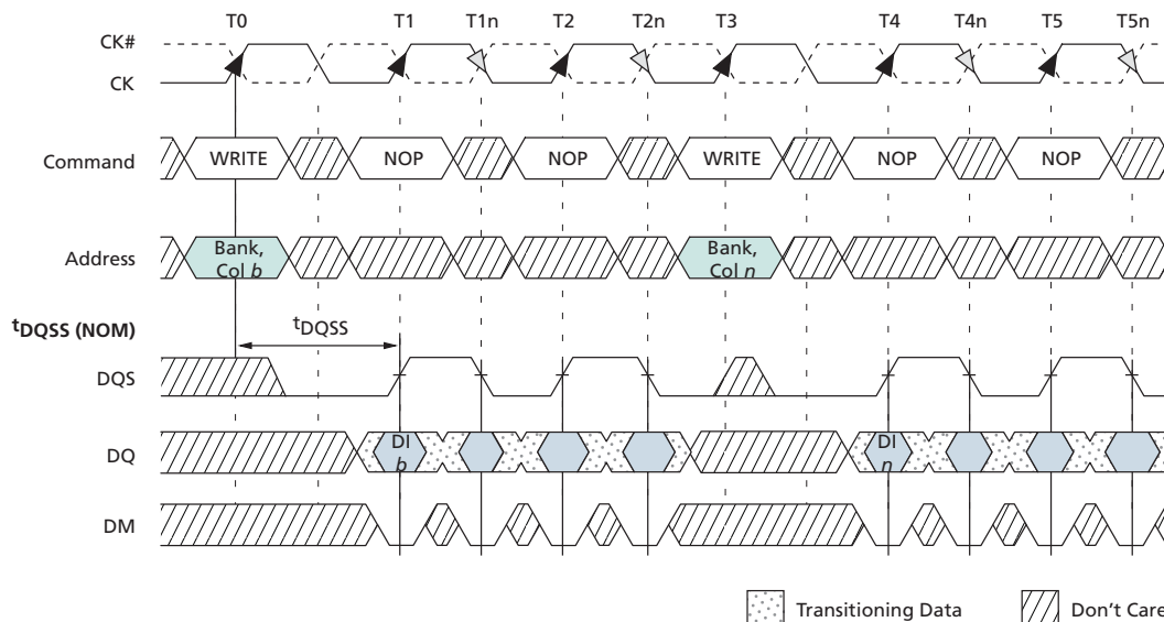
Figure 38: Nonconsecutive WRITE-to-WRITE
