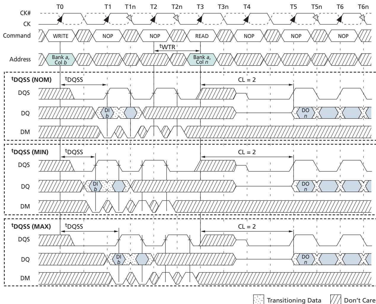
Figure 41: WRITE-to-READ – Interrupting
