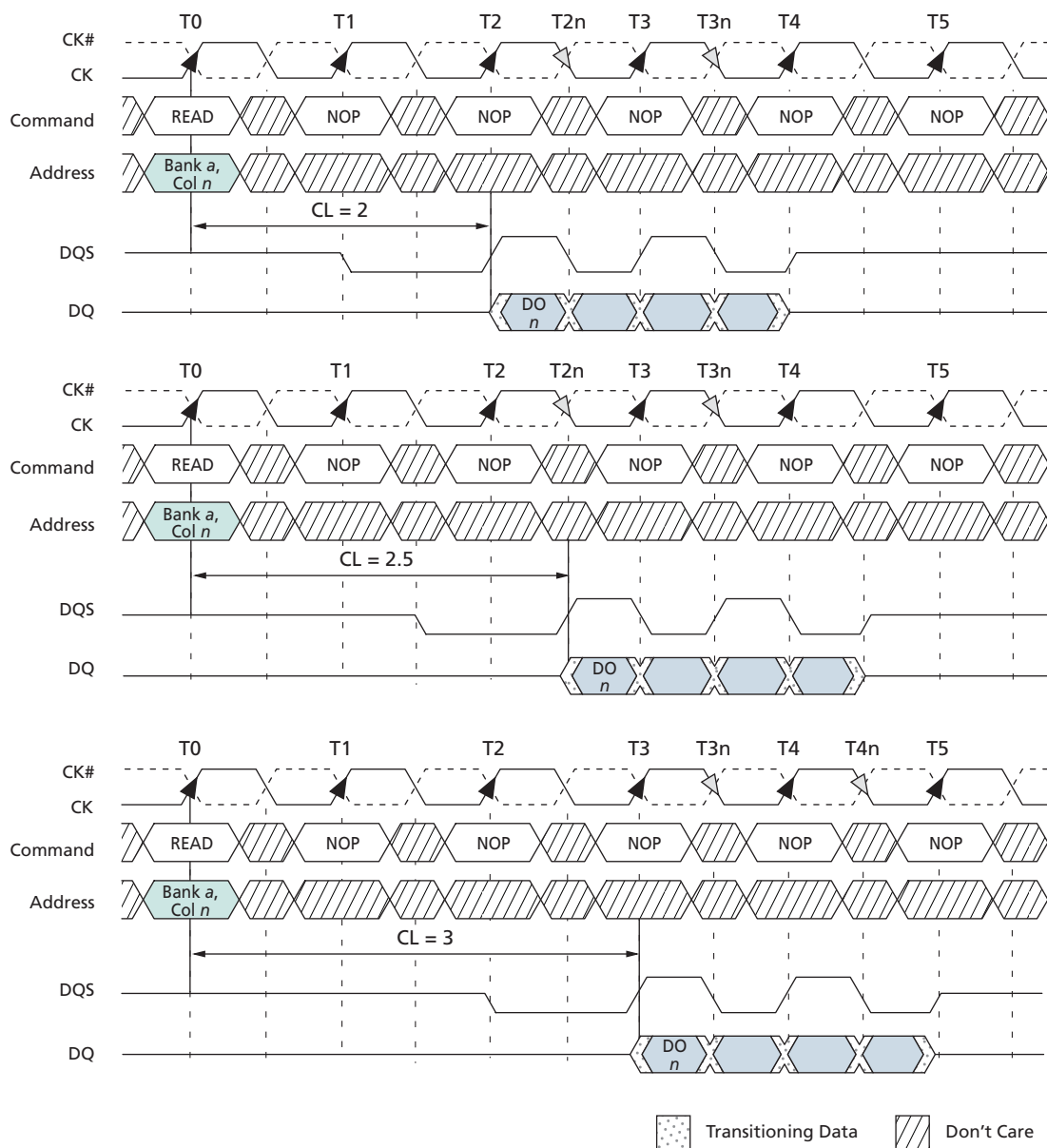
Figure 25: READ Burst
