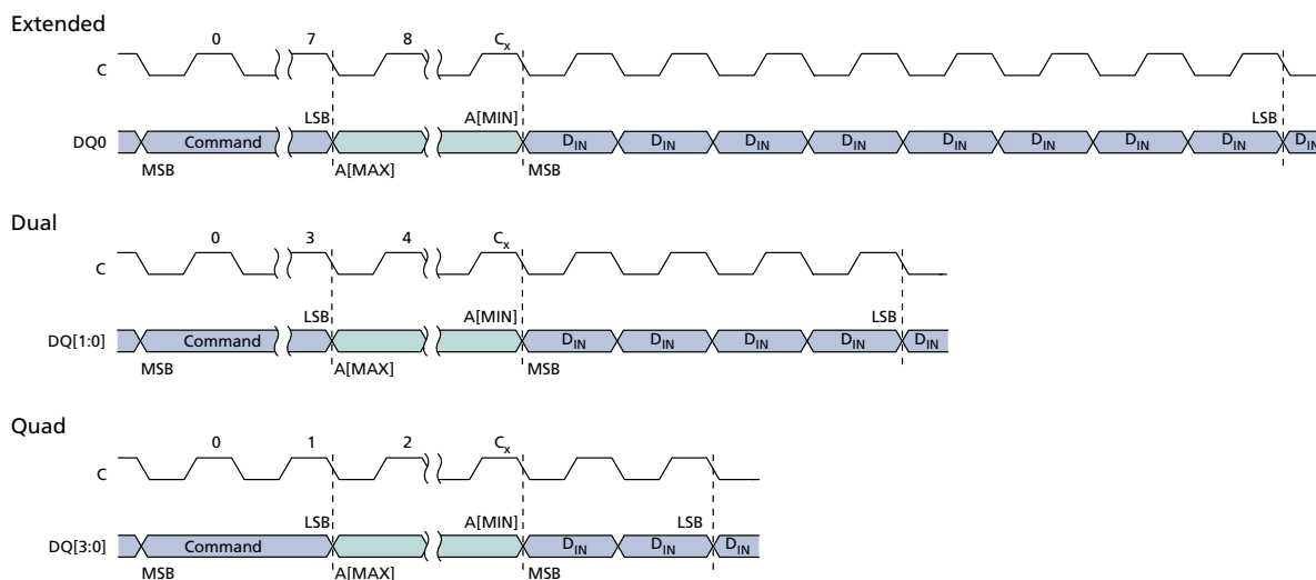
Figure 19: PAGE PROGRAM Command
