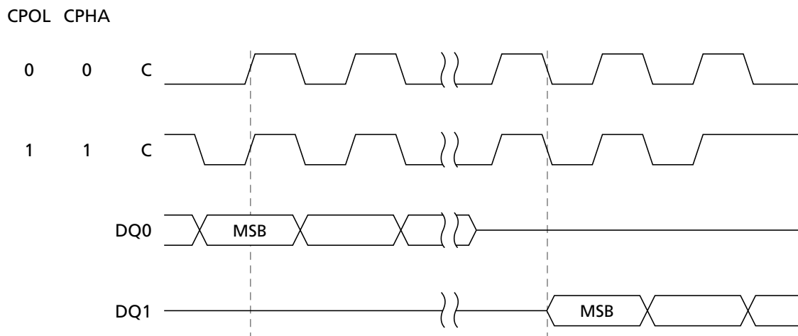
Figure 6: SPI Modes
