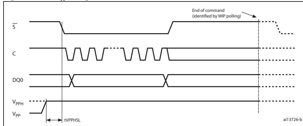
Figure 107. V_{\text{PPH}} timing
