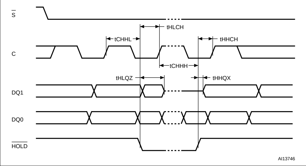
Figure 105. Hold timing
