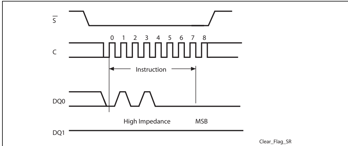
Figure 35. Clear Flag Status Register instruction sequence
