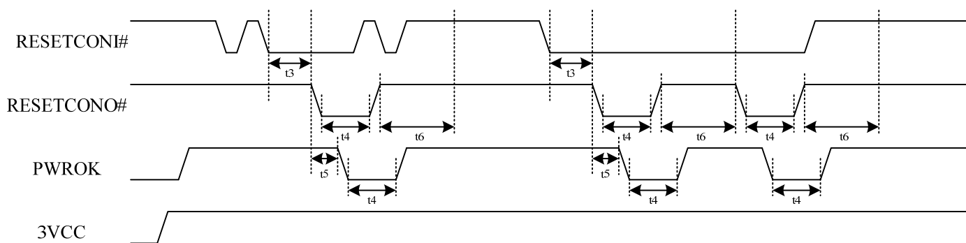
Figure 6-3 RESETCONI# and PWROK
