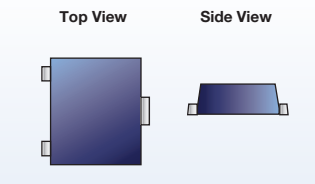
M53 Package (1.0 x 1.2 x 0.33)
