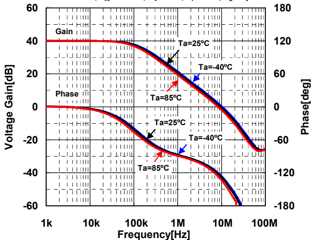
40dB Gain/Phase vs. Frequency (Temperature) V + /V - =±2.5V, V IN =-30dBm, G v =40dB, R F =10kΩ, C L =10pF
