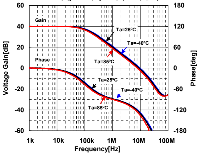
40dB Gain/Phase vs. Frequency (Temperature) V + /V - =±1.25V, V IN =-30dBm, G v =40dB, R F =10kΩ, C L =10pF
