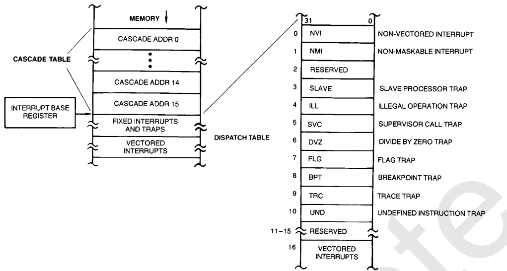
FIGURE 3-4. Interrupt Dispatch and Cascade Tables
