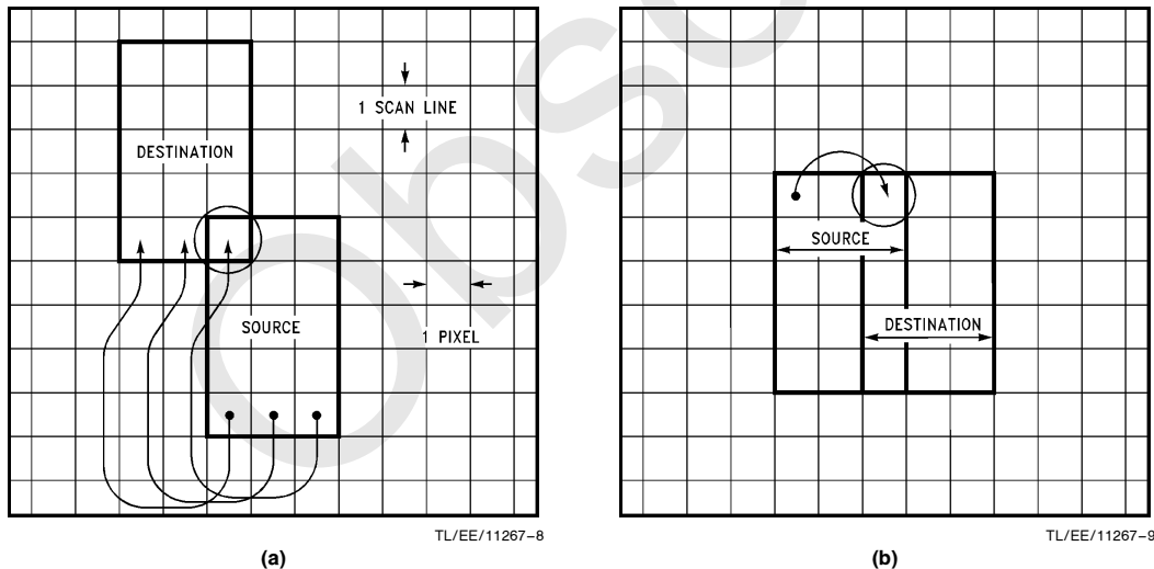
FIGURE 2-22. Overlapping BITBLT Blocks
