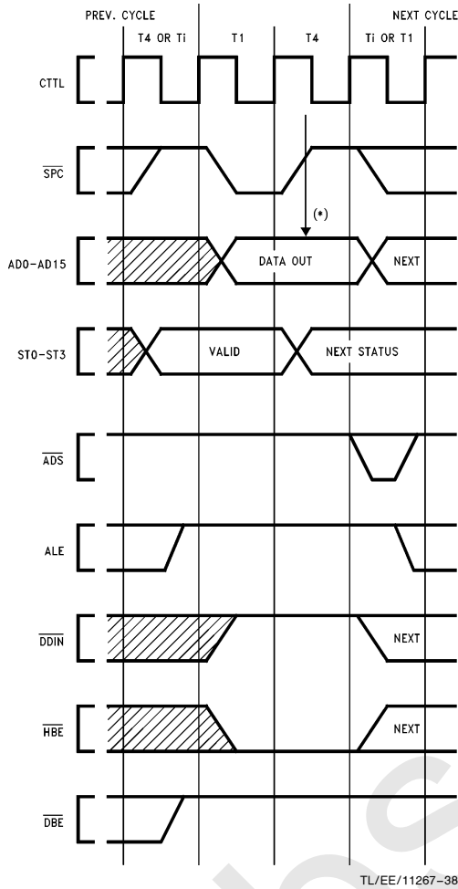
*Note: Slave Processor samples Data Bus here. FIGURE 3-26. Slave Processor Write Cycle 3.5.5.8 Data Access Sequences
