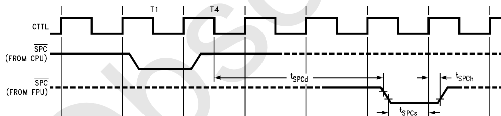
FIGURE 4-12. \overline{\text{SPC}} Timing
