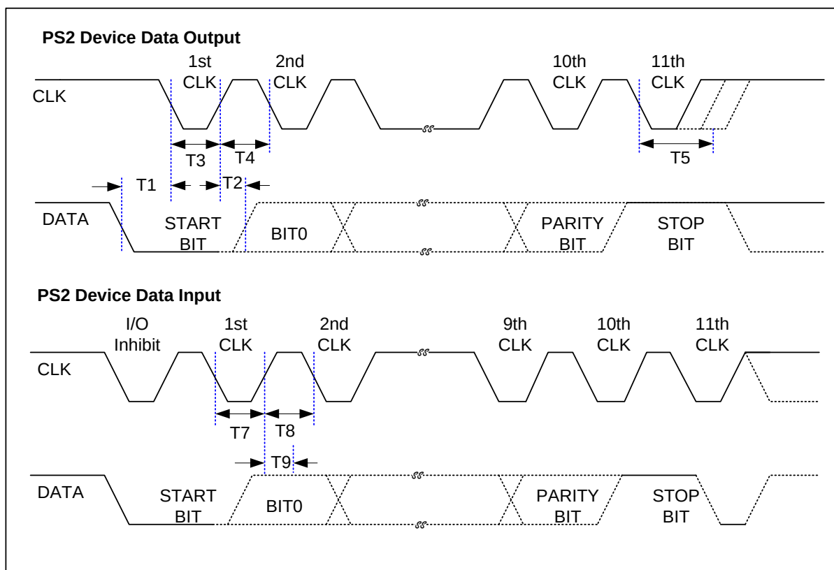
Figure 5-91 PS/2 Bus Timing
