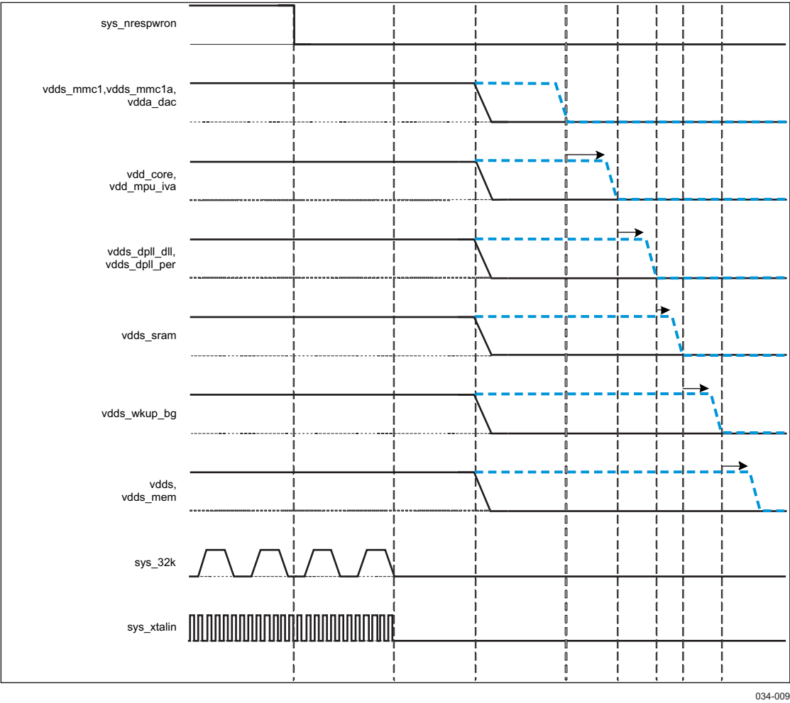
Figure 3-4. Power-down Sequence
