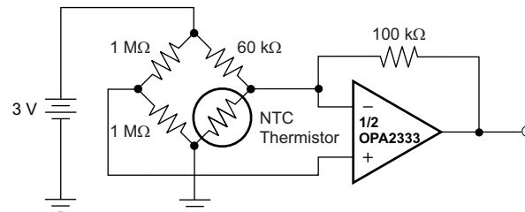
Figure 33. Thermistor Measurement
