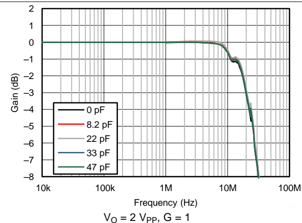
Figure 6. Large-Signal Frequency Response for Various Capacitive Loads
