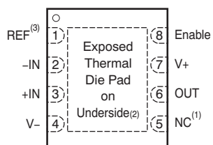
OPA728 DFN-8 (TOP VIEW)
