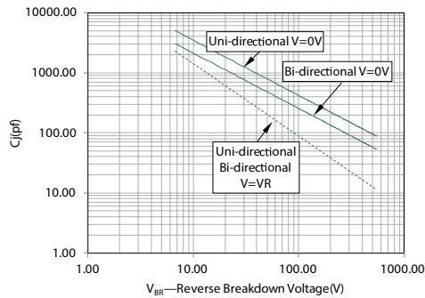
Figure 5 - Typical Junction Capacitance
