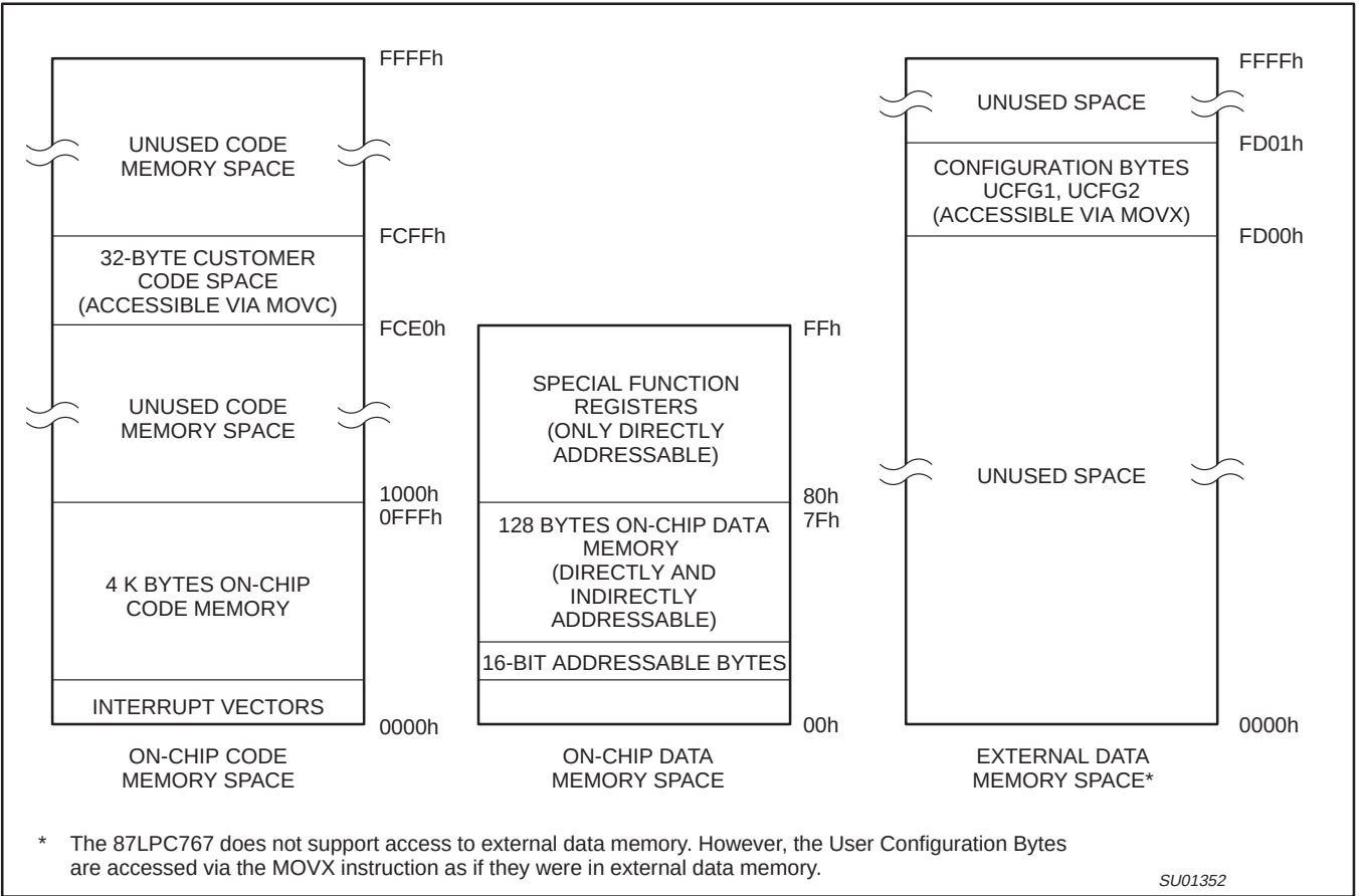
Figure 1. P87LPC767 Program and Data Memory Map
