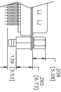
TERMINATION-MTG. OPTION 2.32 VERTICAL MOUNT, #4-40 UNC HEX JACK SOCKETS, STANDOFFS WITH BOARDLOCKS
