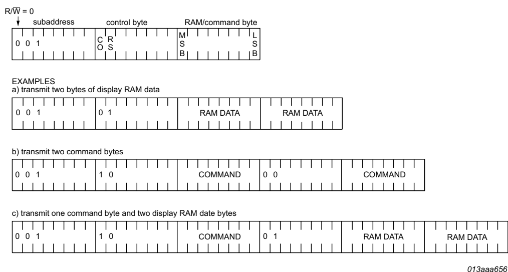
Fig 49. SPI-bus write example
