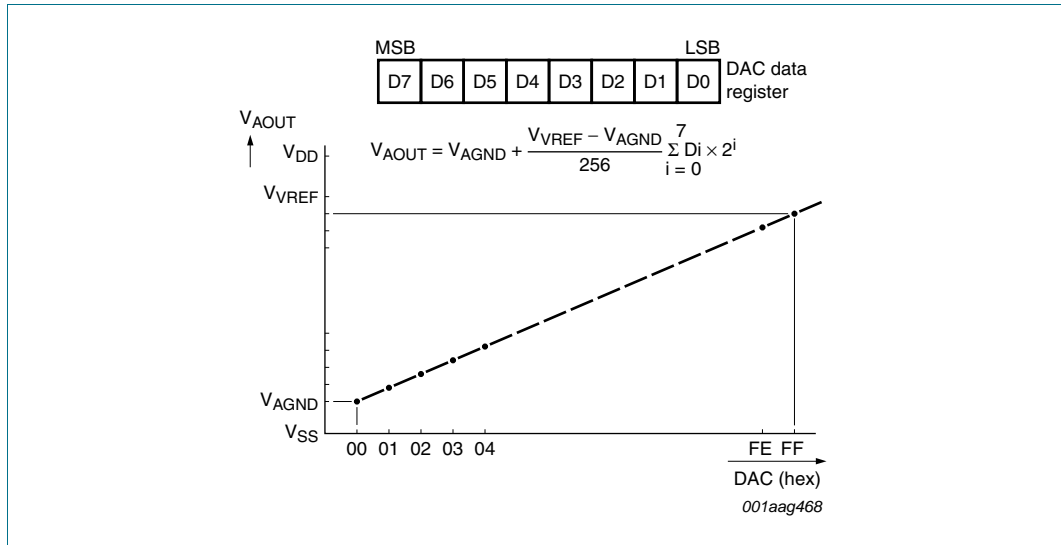
Fig 8. DAC data and DC conversion characteristics
