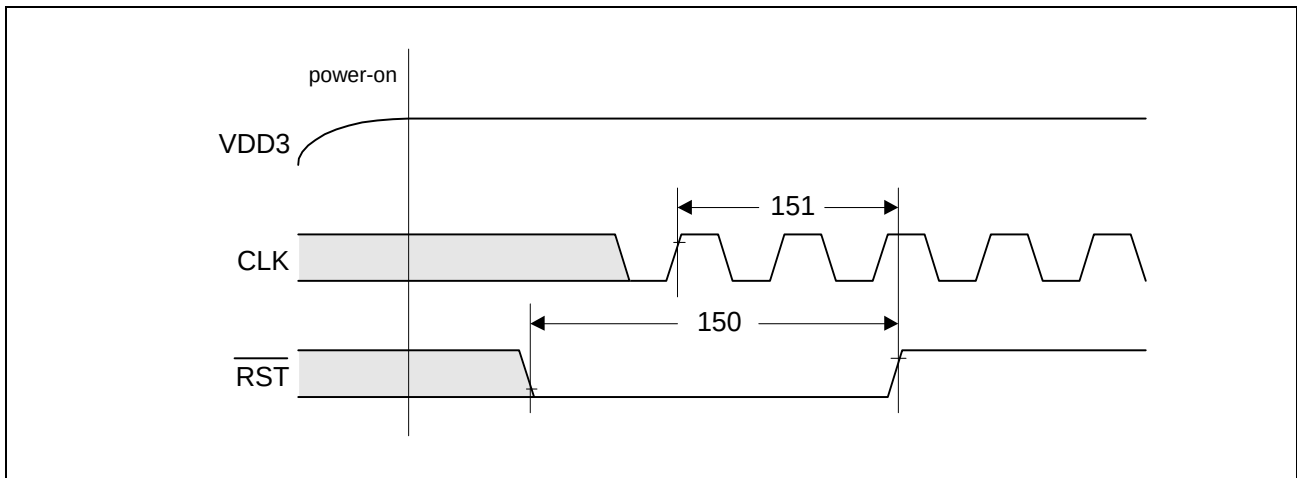
Figure 106 Reset Timing
