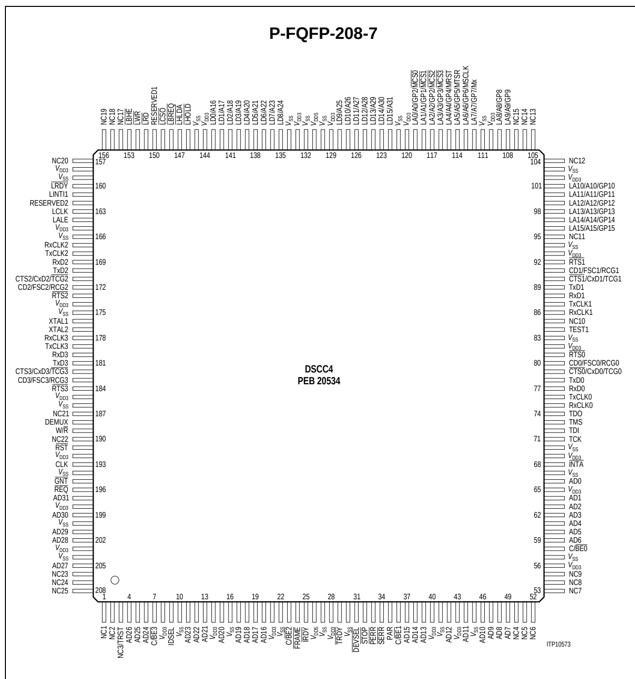
Figure 7 Pin Configuration
