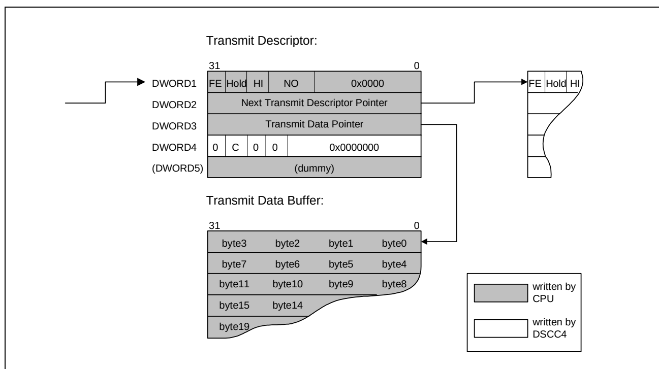
Figure 77 Transmit Descriptor List Structure
