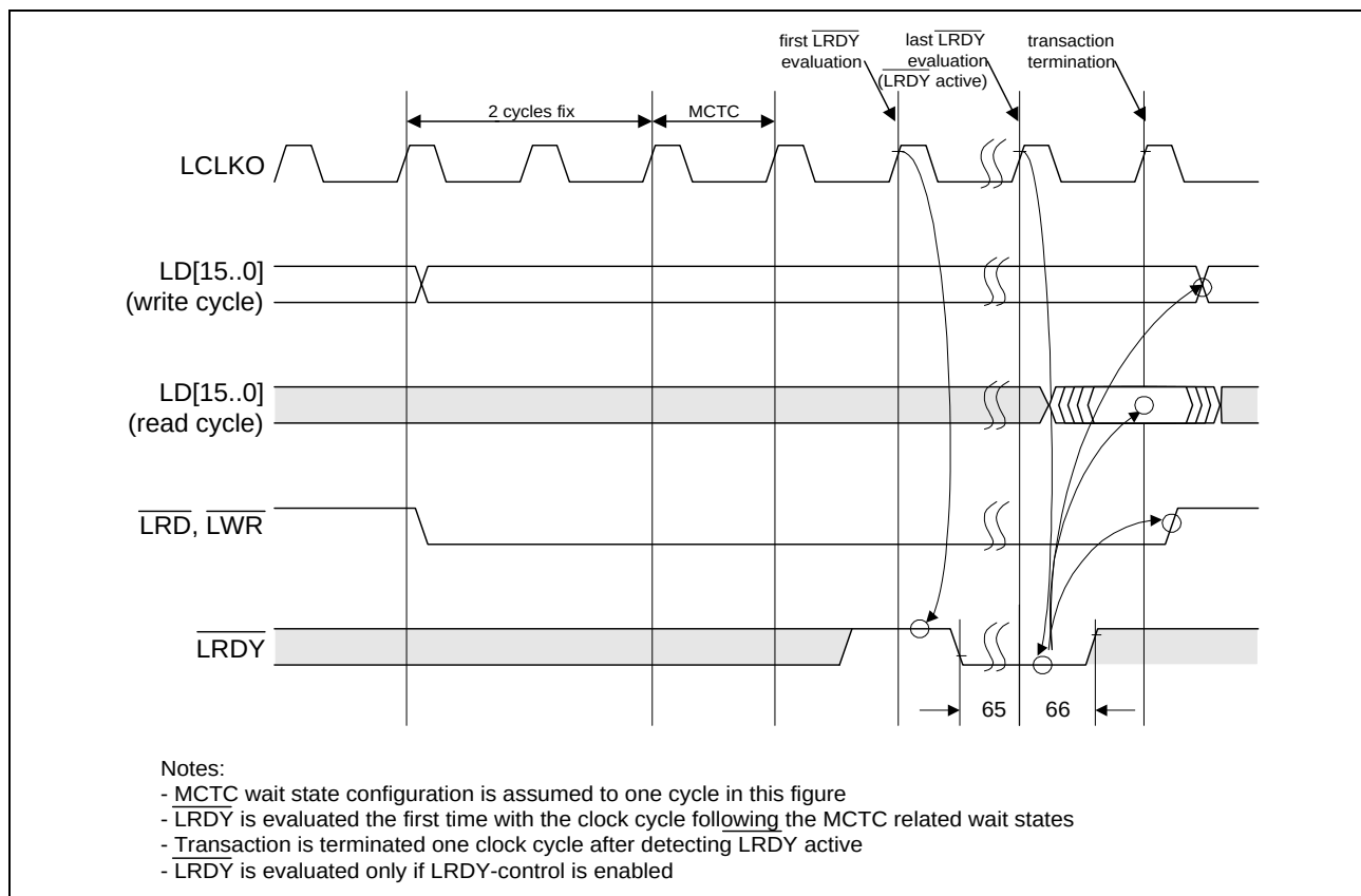
Figure 97 \overline{\text{LRDY}} Timing
