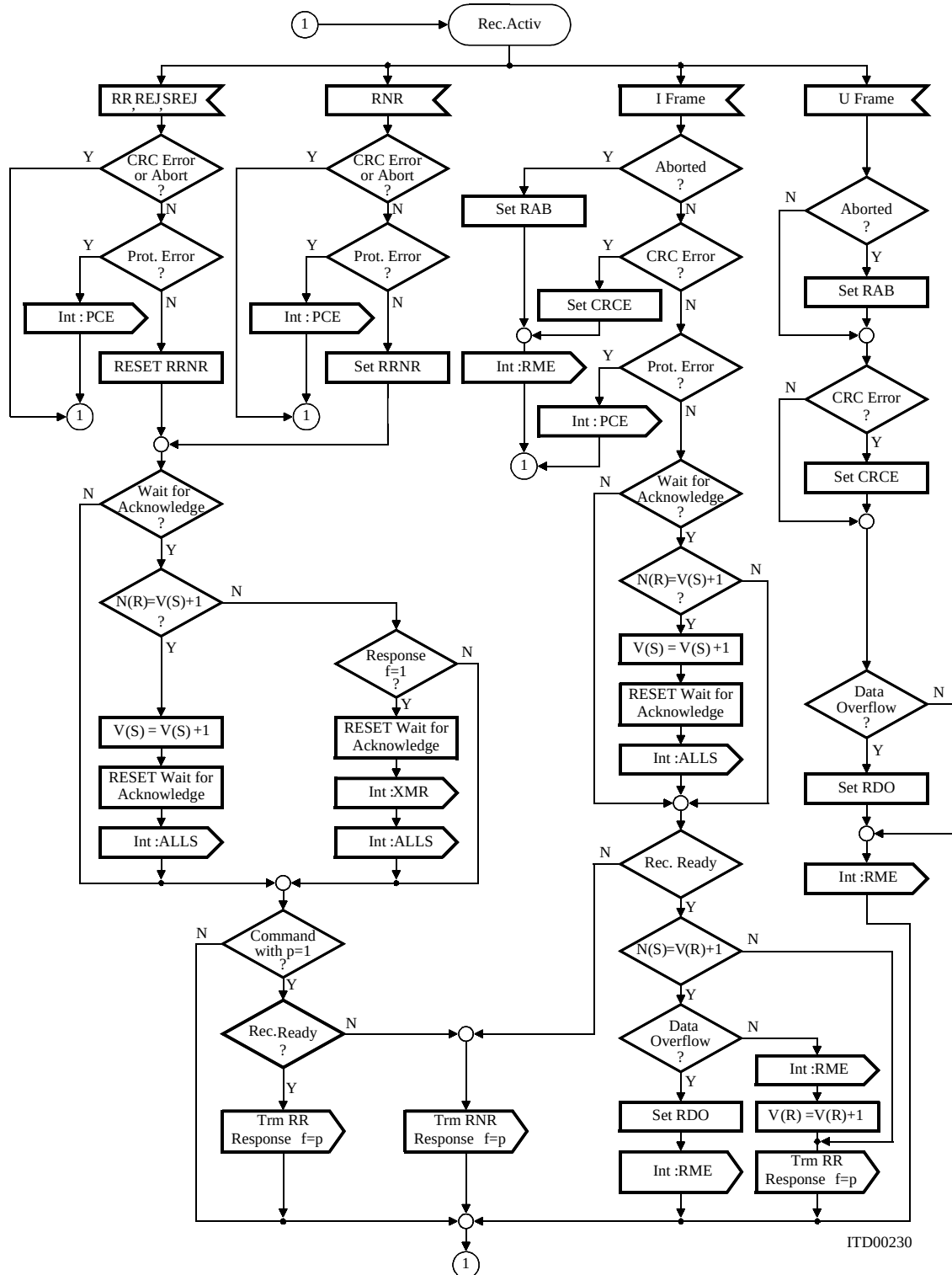
Figure 64 Processing of Received Frames in Auto Mode
