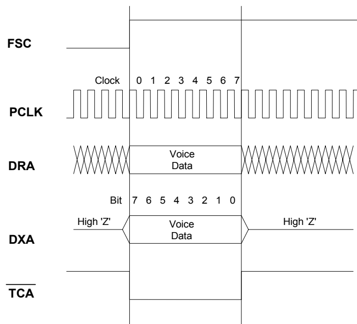
Figure 52 General PCM Interface Timing
