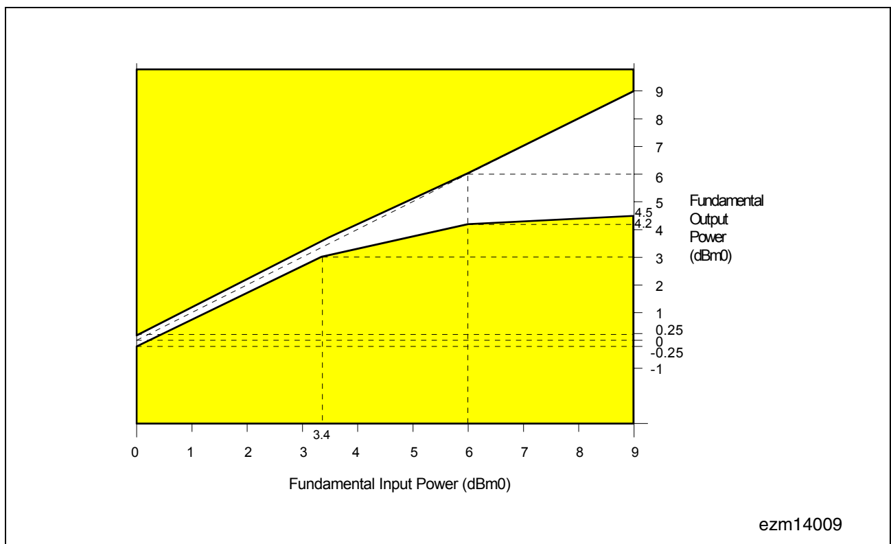
Figure 72 Overload Compression
