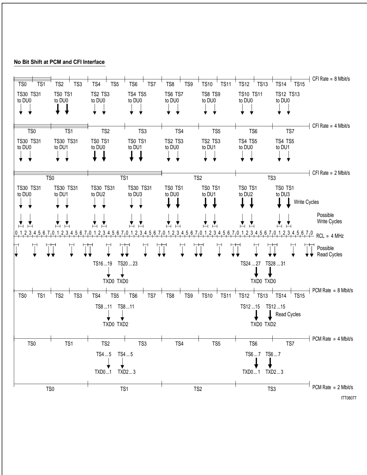
Figure 62 Internal Timing Data Upstream
