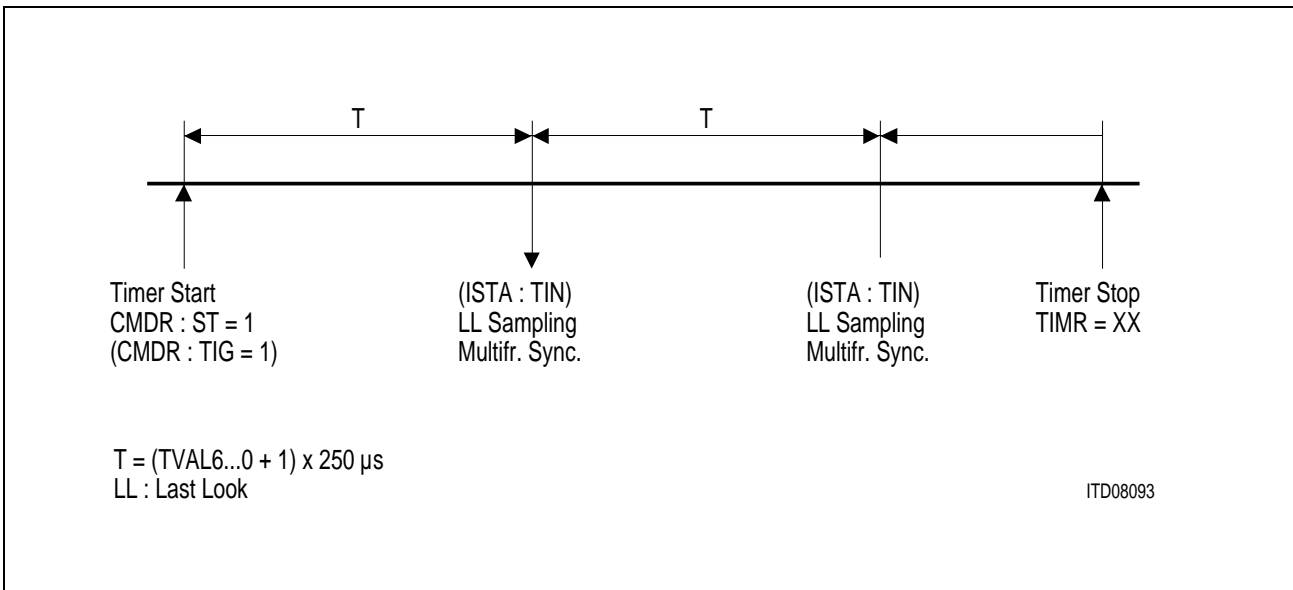
Figure 77 Timer Applications
