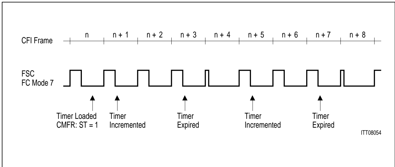
Figure 39 FSC Signal in FC Mode 7
