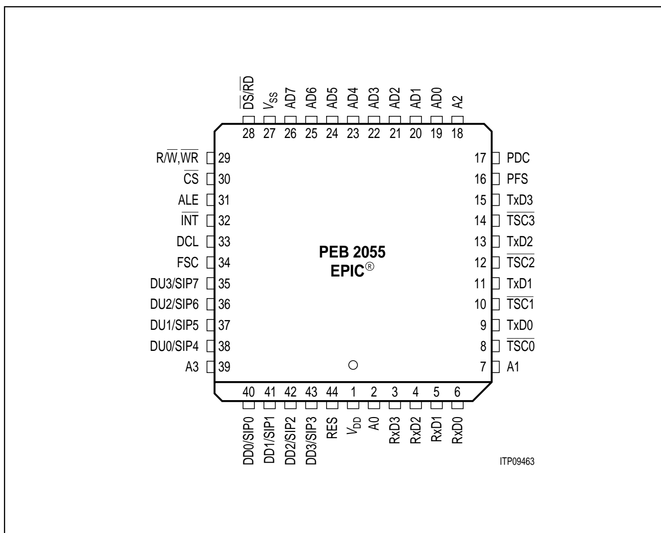
Figure 1 Pin Configuration EPIC®-1
