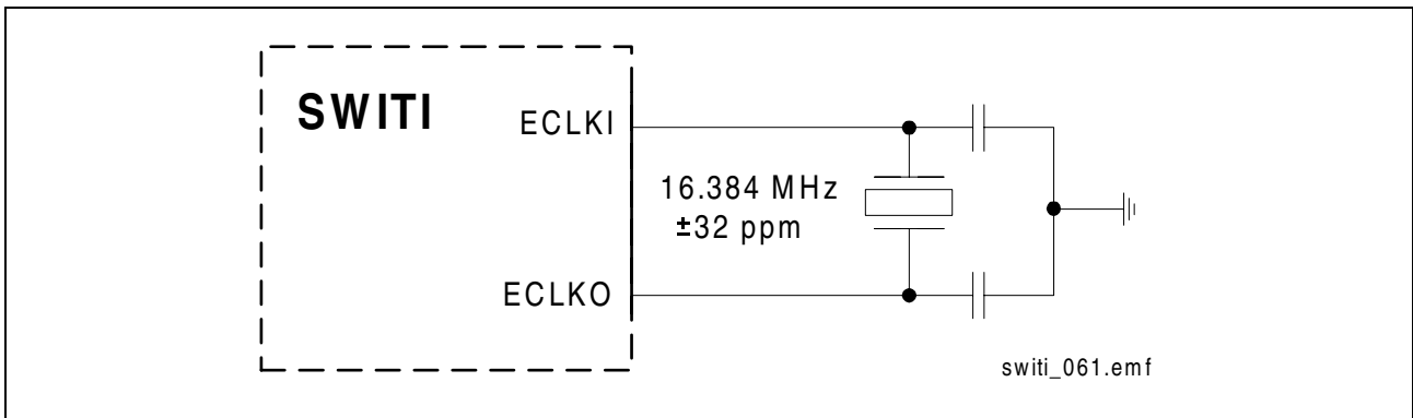
Figure 59 External Crystal
