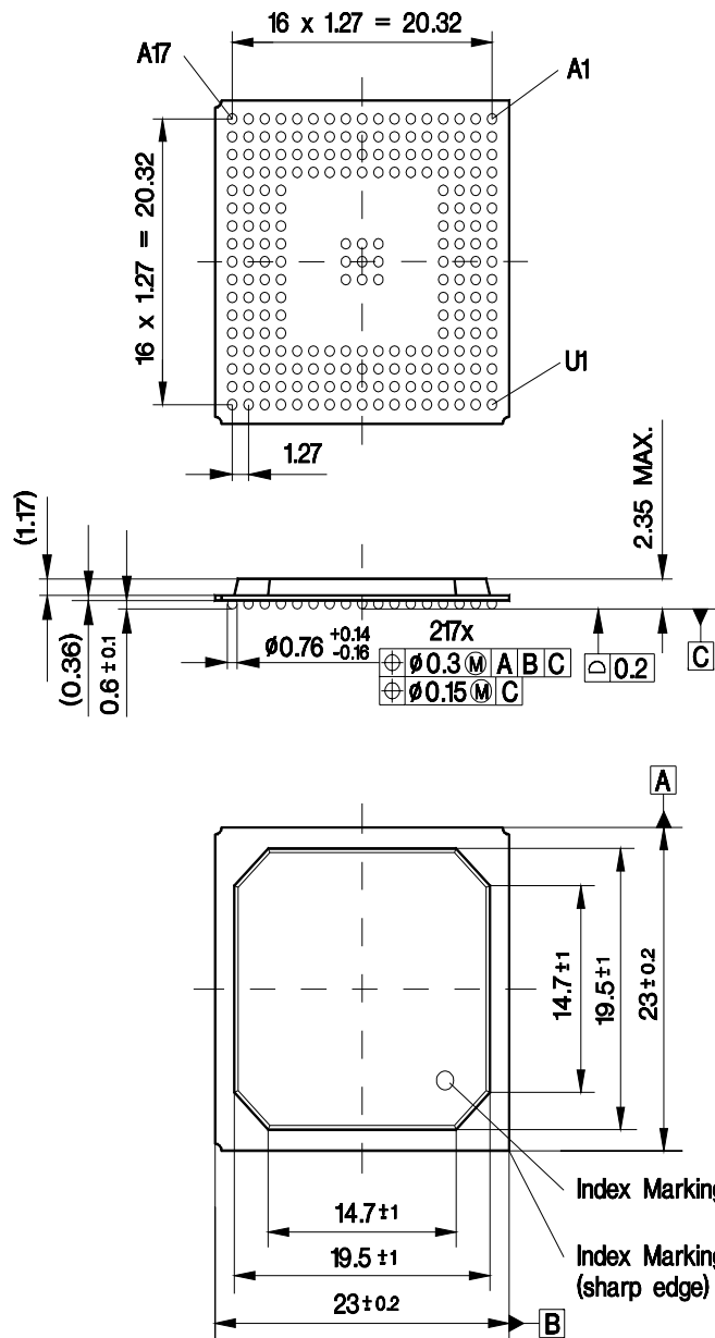
Figure 61 Outlines of P-BGA-217-1
