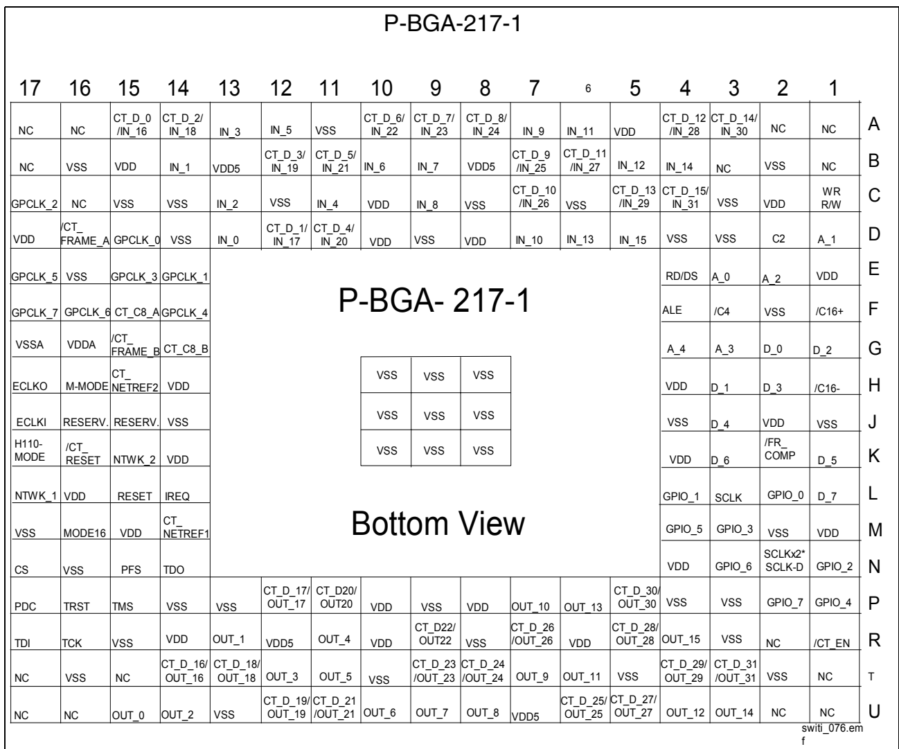
Figure 7 Pin Configuration
