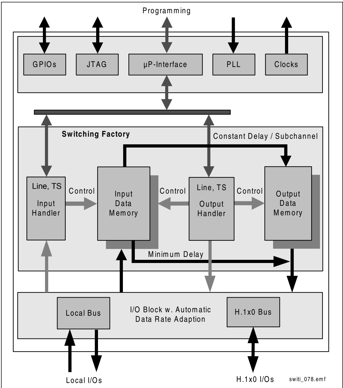
Figure 8 Block Diagram
