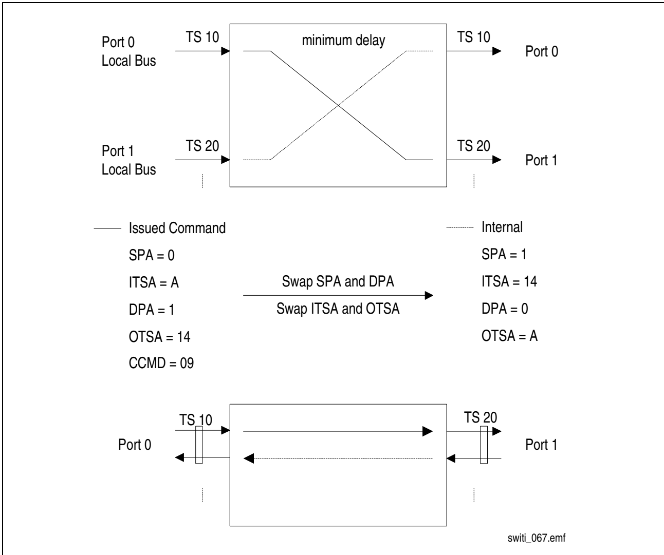
Figure 9 Bidirectional Mode
