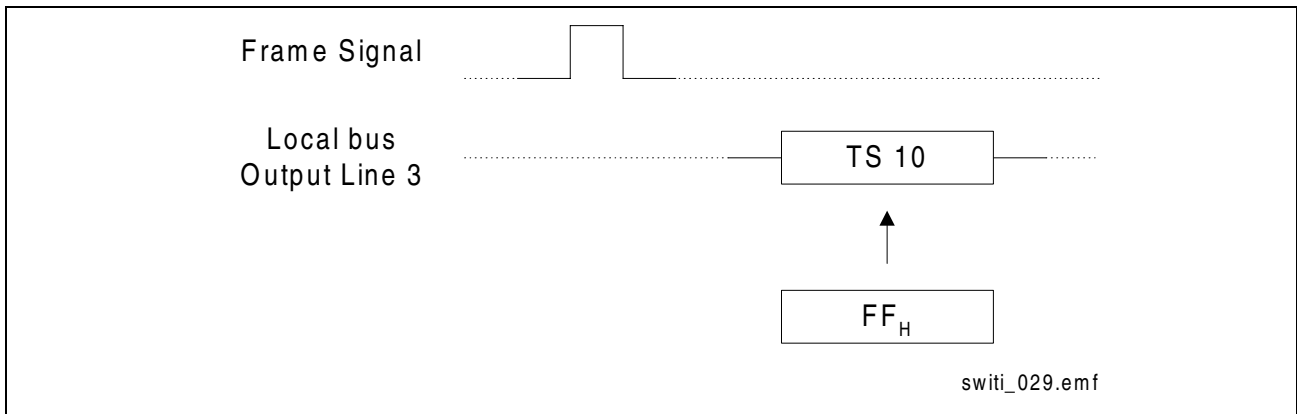
Figure 41 Example: Send Message
