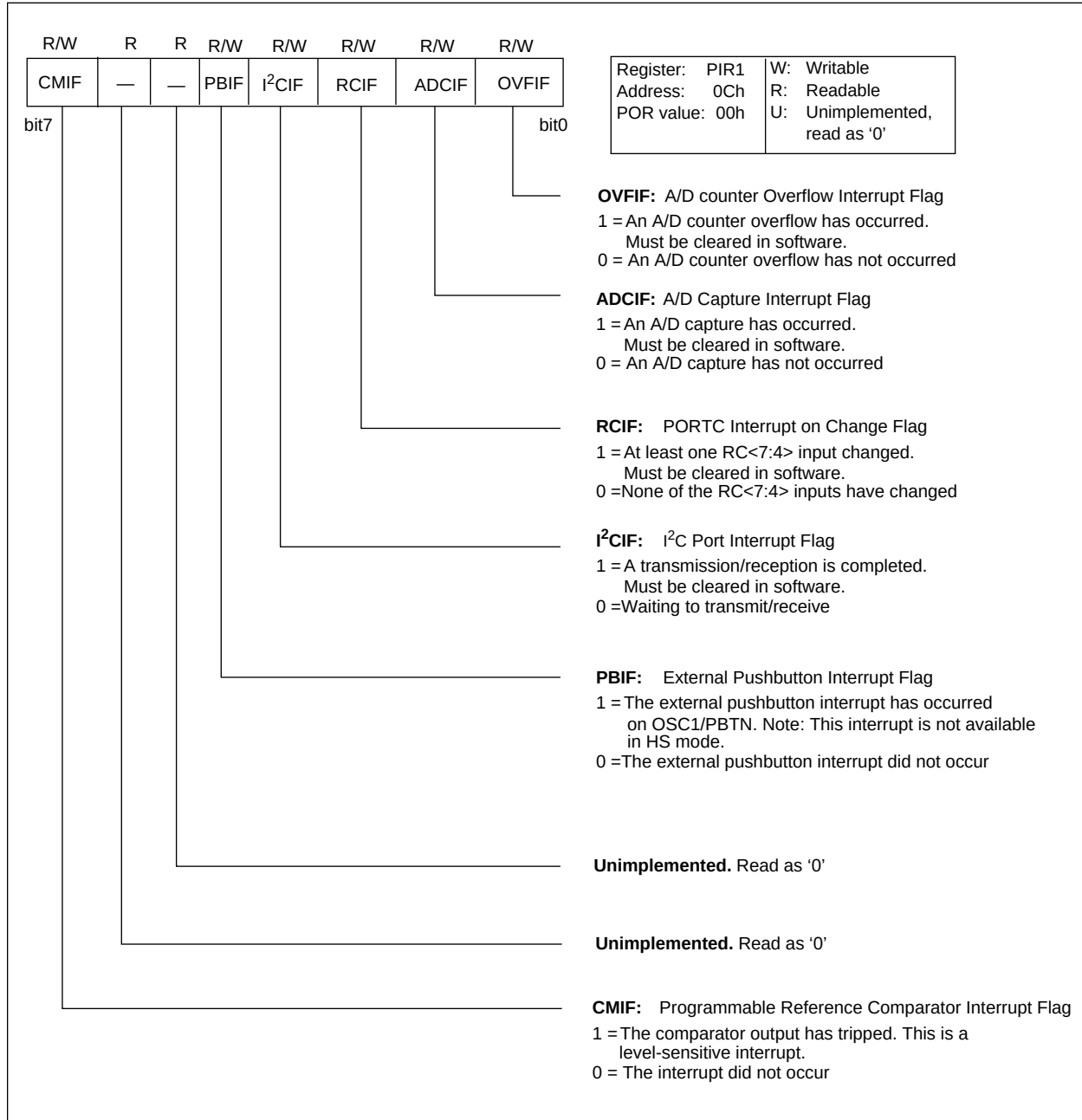
FIGURE 4-7: PIR1 REGISTER
