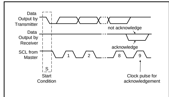
FIGURE 7-6: I 2 C SLAVE-RECEIVER ACKNOWLEDGE
