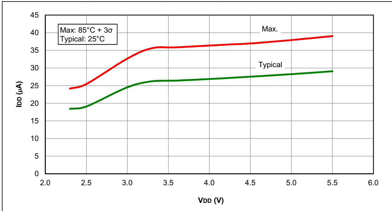
FIGURE 26-2: I_{DD} , LP OSCILLATOR, F_{osc} = 32 kHz, PIC16F1526/7 ONLY
