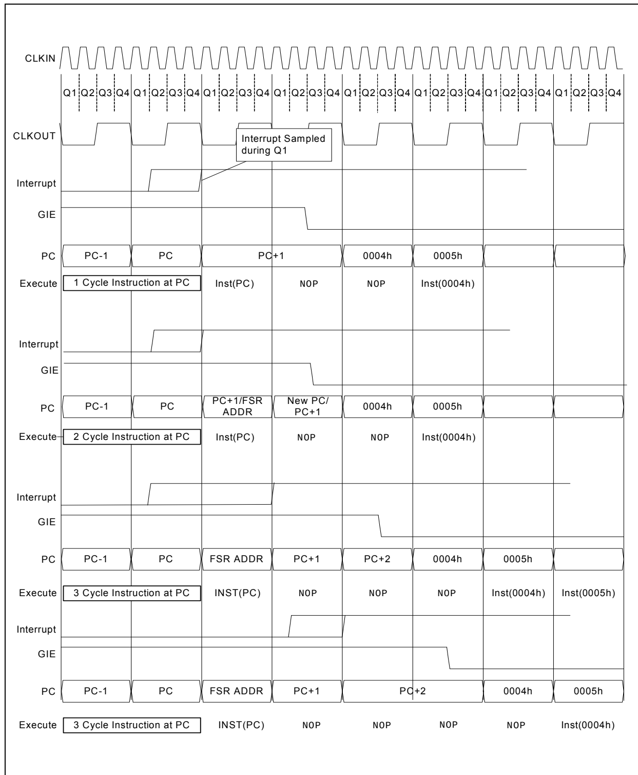
FIGURE 7-2: INTERRUPT LATENCY
