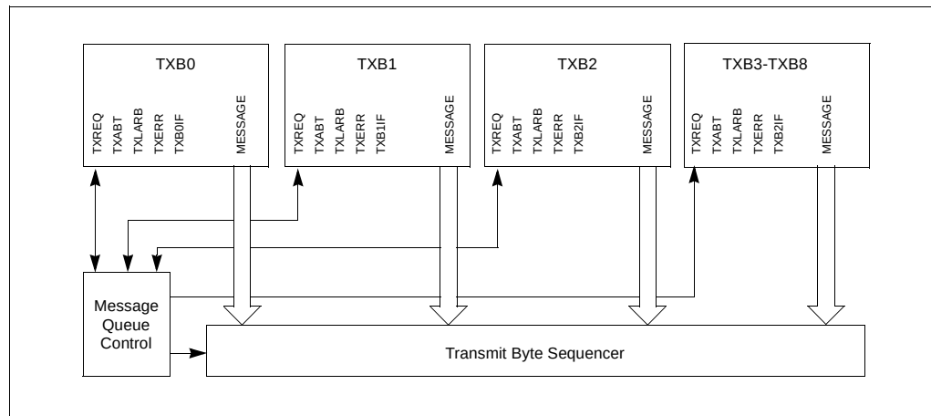
FIGURE 23-2: TRANSMIT BUFFERS
