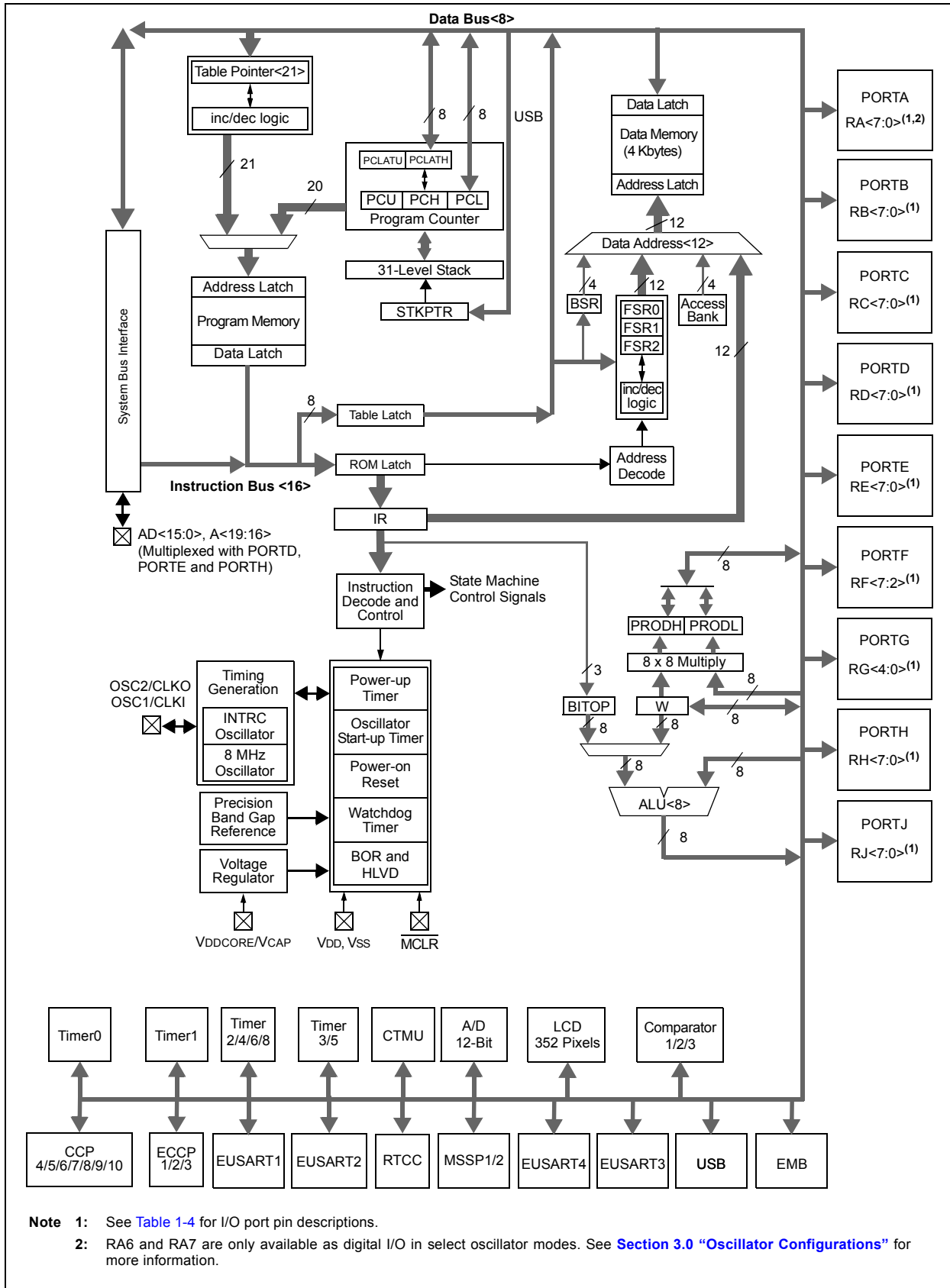
FIGURE 1-2: 80-PIN DEVICE BLOCK DIAGRAM
