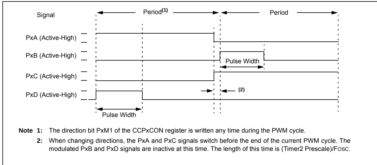
FIGURE 15-12: EXAMPLE OF PWM DIRECTION CHANGE
