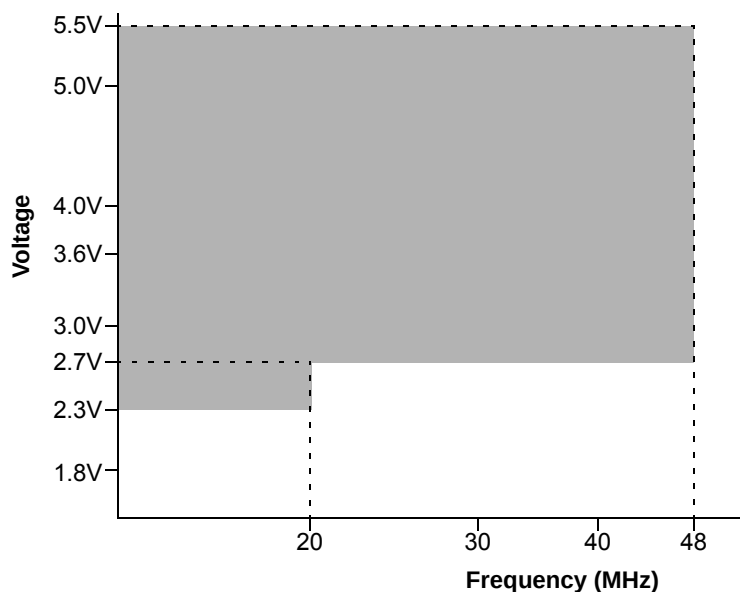
FIGURE 29-2: PIC18F2X/45K50 FAMILY VOLTAGE-FREQUENCY GRAPH (INDUSTRIAL TEMPERATURE)
