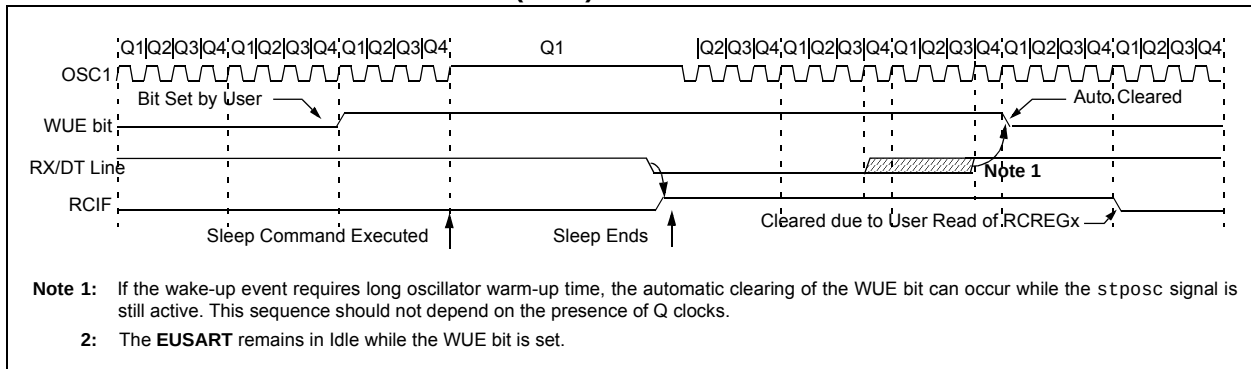
FIGURE 17-8: AUTO-WAKE-UP BIT (WUE) TIMINGS DURING SLEEP
