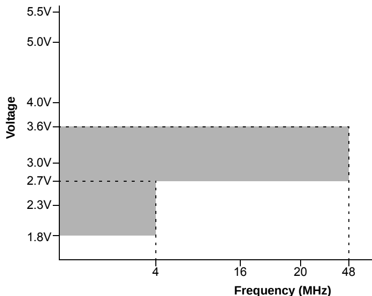
FIGURE 29-1: PIC18LF2X/45K50 FAMILY VOLTAGE-FREQUENCY GRAPH (INDUSTRIAL AND EXTENDED TEMPERATURE)
