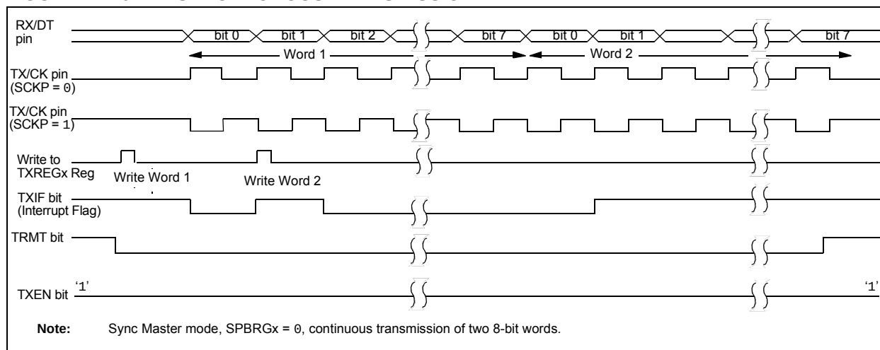
FIGURE 17-10: SYNCHRONOUS TRANSMISSION
