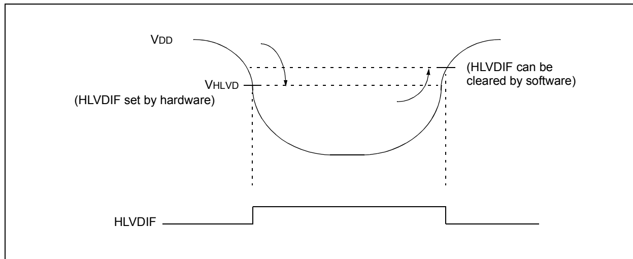
FIGURE 29-4: HIGH/LOW-VOLTAGE DETECT CHARACTERISTICS
