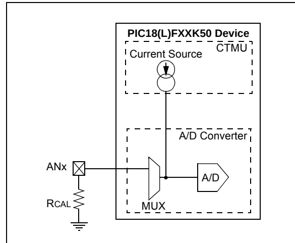
FIGURE 20-2: CTMU CURRENT SOURCE CALIBRATION CIRCUIT
