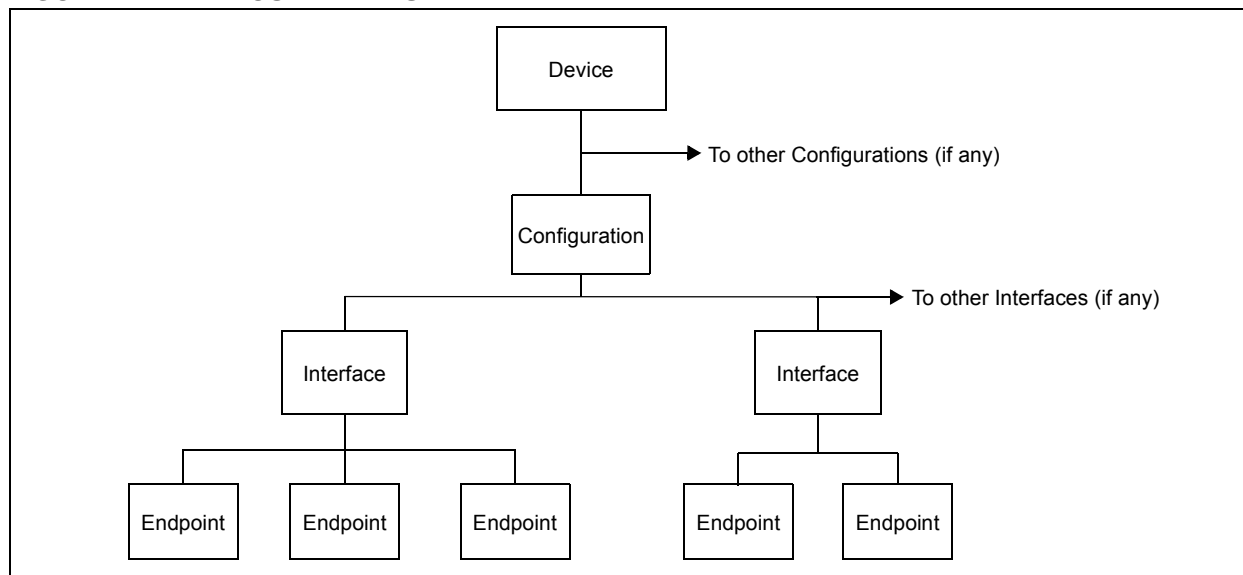
FIGURE 24-12: USB LAYERS
