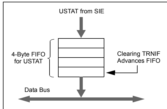
FIGURE 24-3: USTAT FIFO
