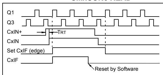
FIGURE 19-3: COMPARATOR INTERRUPT TIMING W/O CMxCON0 READ
