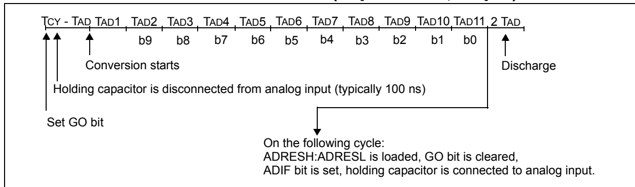
FIGURE 18-3: A/D CONVERSION TAD CYCLES (ACQT<2:0> = 000, TACQ = 0)
