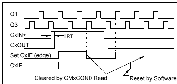
FIGURE 19-4: COMPARATOR INTERRUPT TIMING WITH CMxCON0 READ
