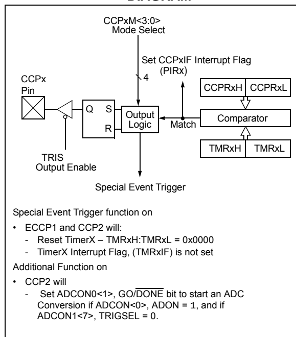
FIGURE 15-2: COMPARE MODE OPERATION BLOCK DIAGRAM
