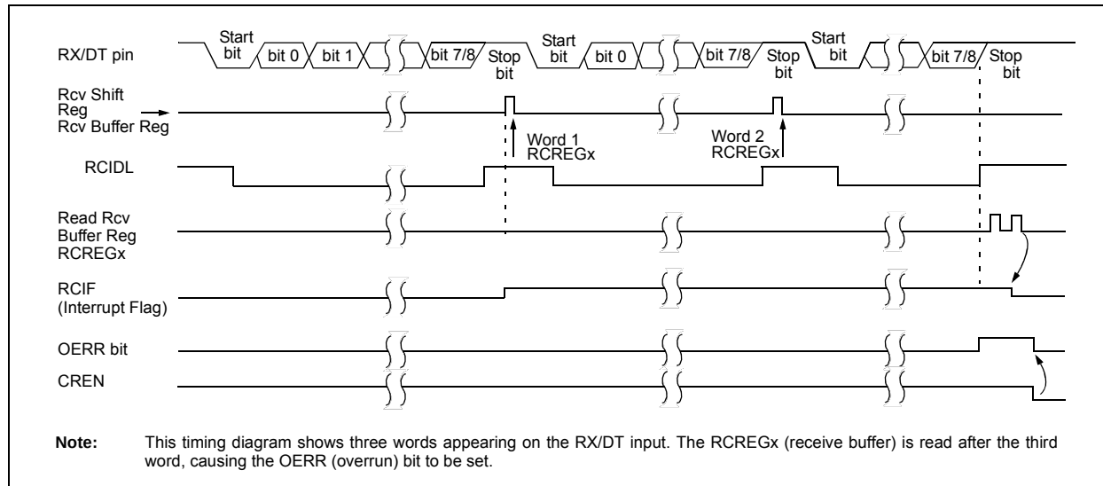
FIGURE 17-5: ASYNCHRONOUS RECEPTION
