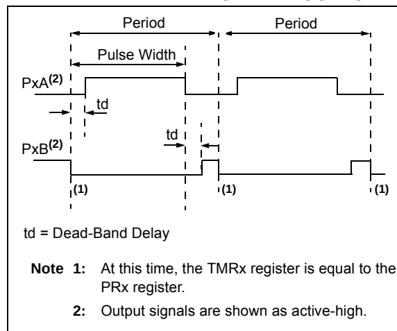
FIGURE 15-16: EXAMPLE OF HALF-BRIDGE PWM OUTPUT
