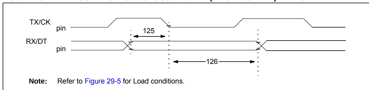
FIGURE 29-21: EUSART SYNCHRONOUS RECEIVE (MASTER/SLAVE) TIMING
