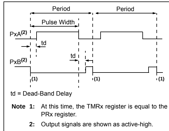
FIGURE 15-8: EXAMPLE OF HALF-BRIDGE PWM OUTPUT
