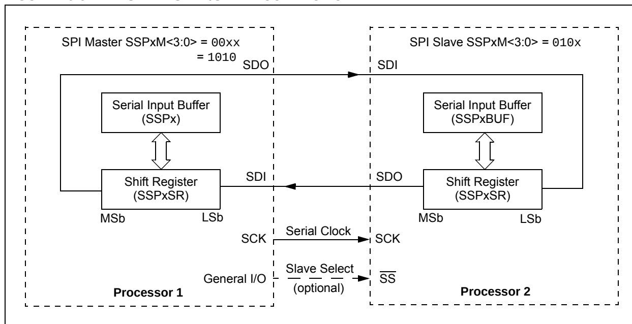
FIGURE 16-5: SPI MASTER/S�AVE CONNECTION
