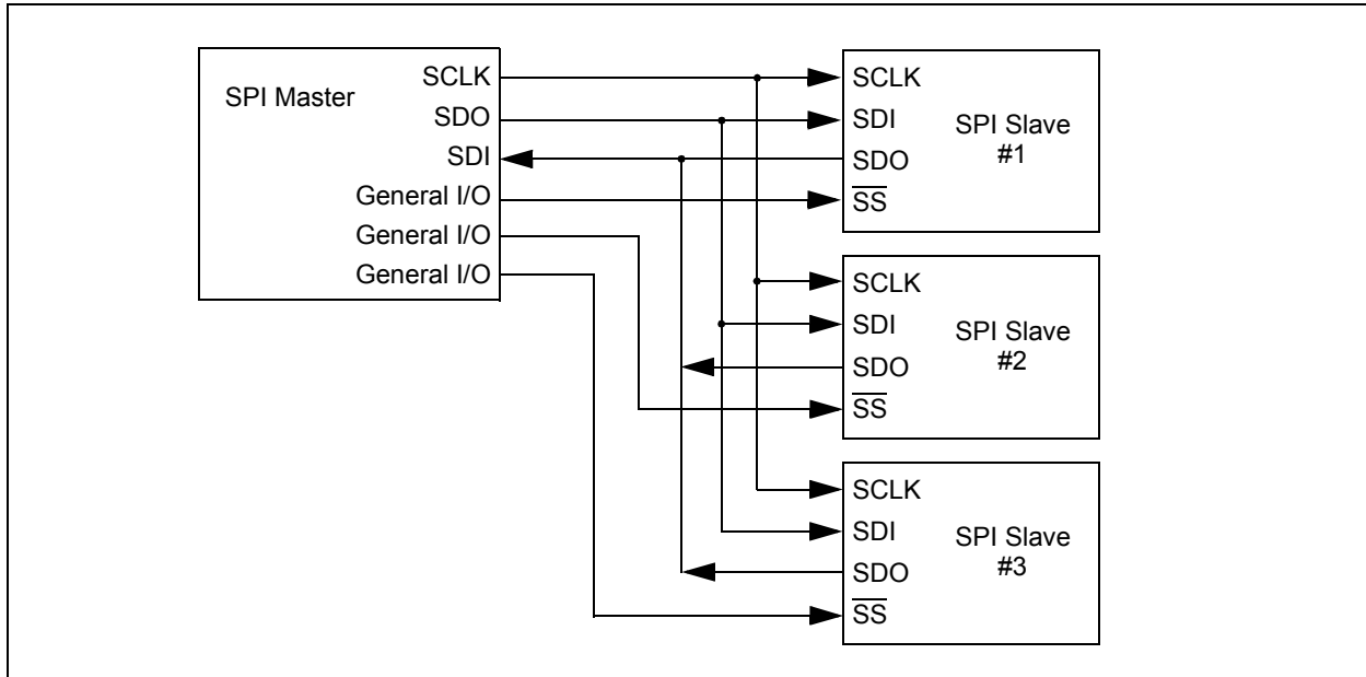
FIGURE 16-4: SPI MASTER AND MULTIPLE SLAVE CONNECTION
