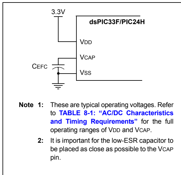
FIGURE 2-2: CONNECTIONS FOR THE ON-CHIP REGULATOR
