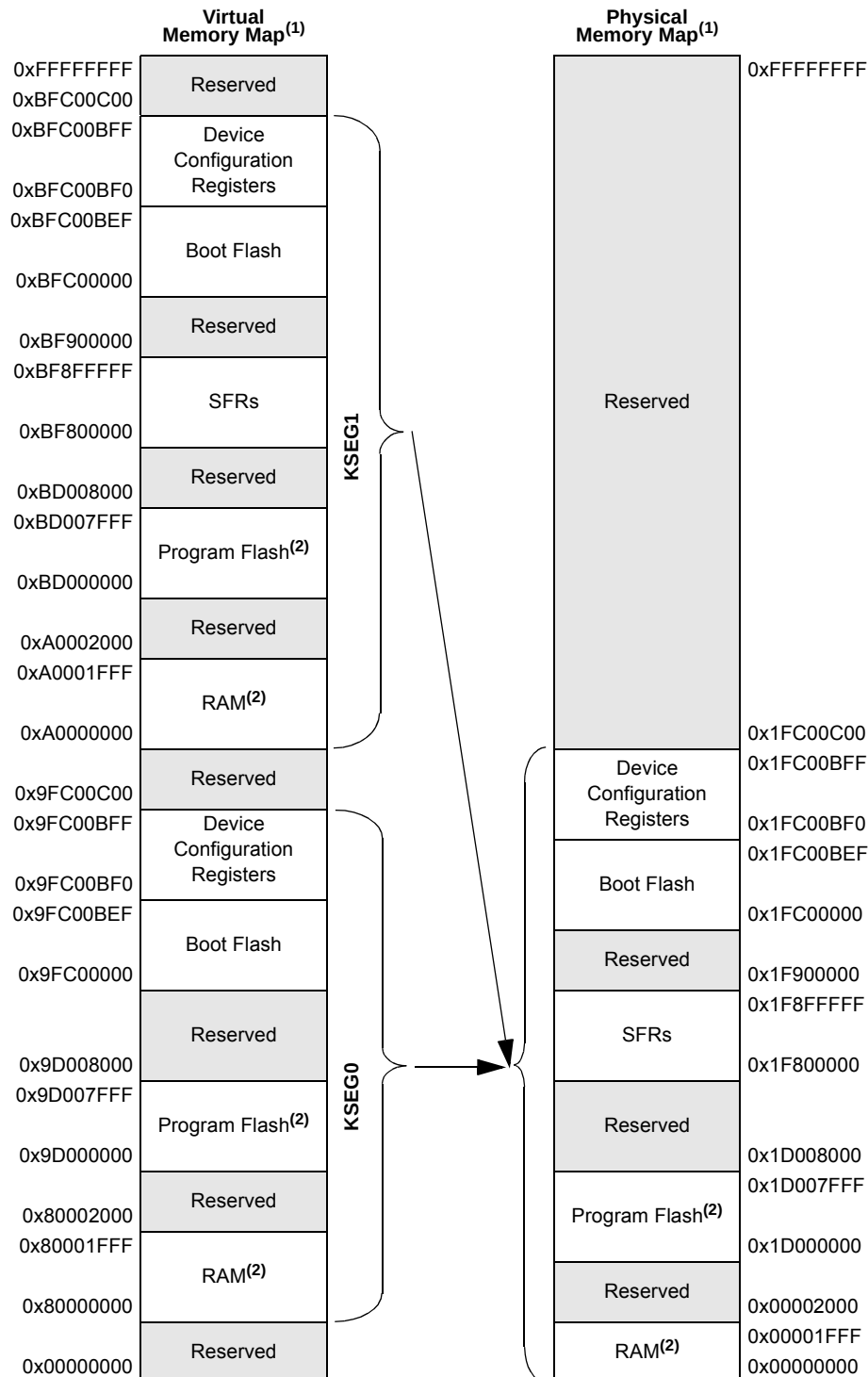
FIGURE 4-2: MEMORY MAP ON RESET FOR PIC32MX120/220 DEVICES (8 KB RAM, 32 KB FLASH)
