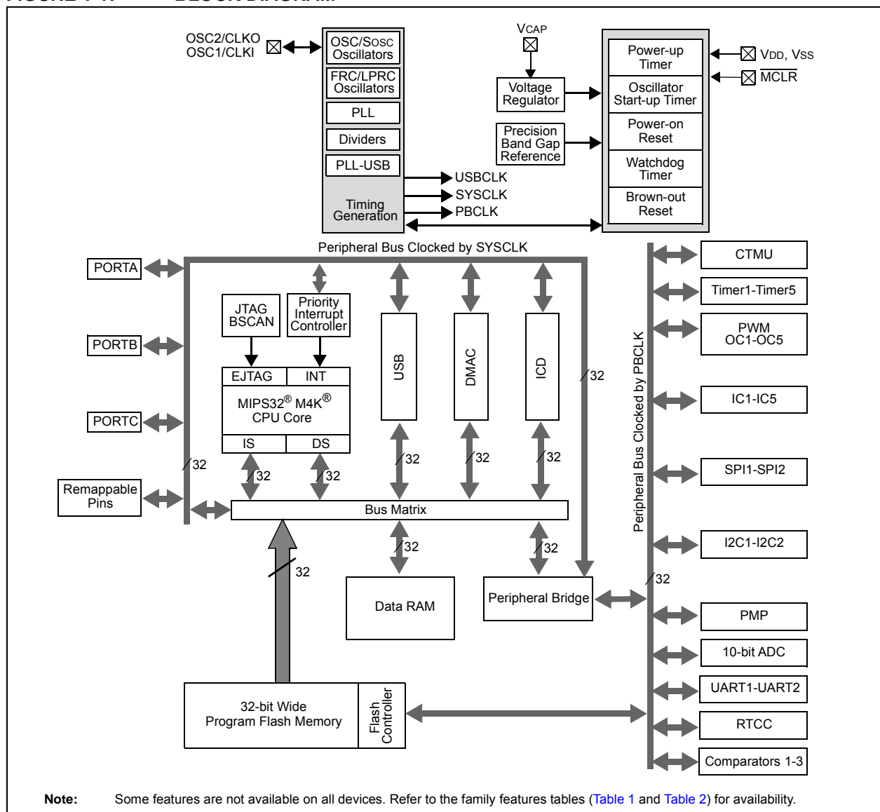
FIGURE 1-1: BLOCK DIAGRAM
