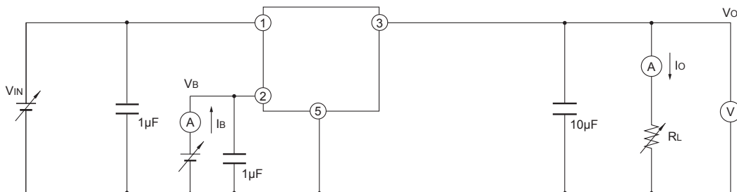
Fig.1 Test Circuit
