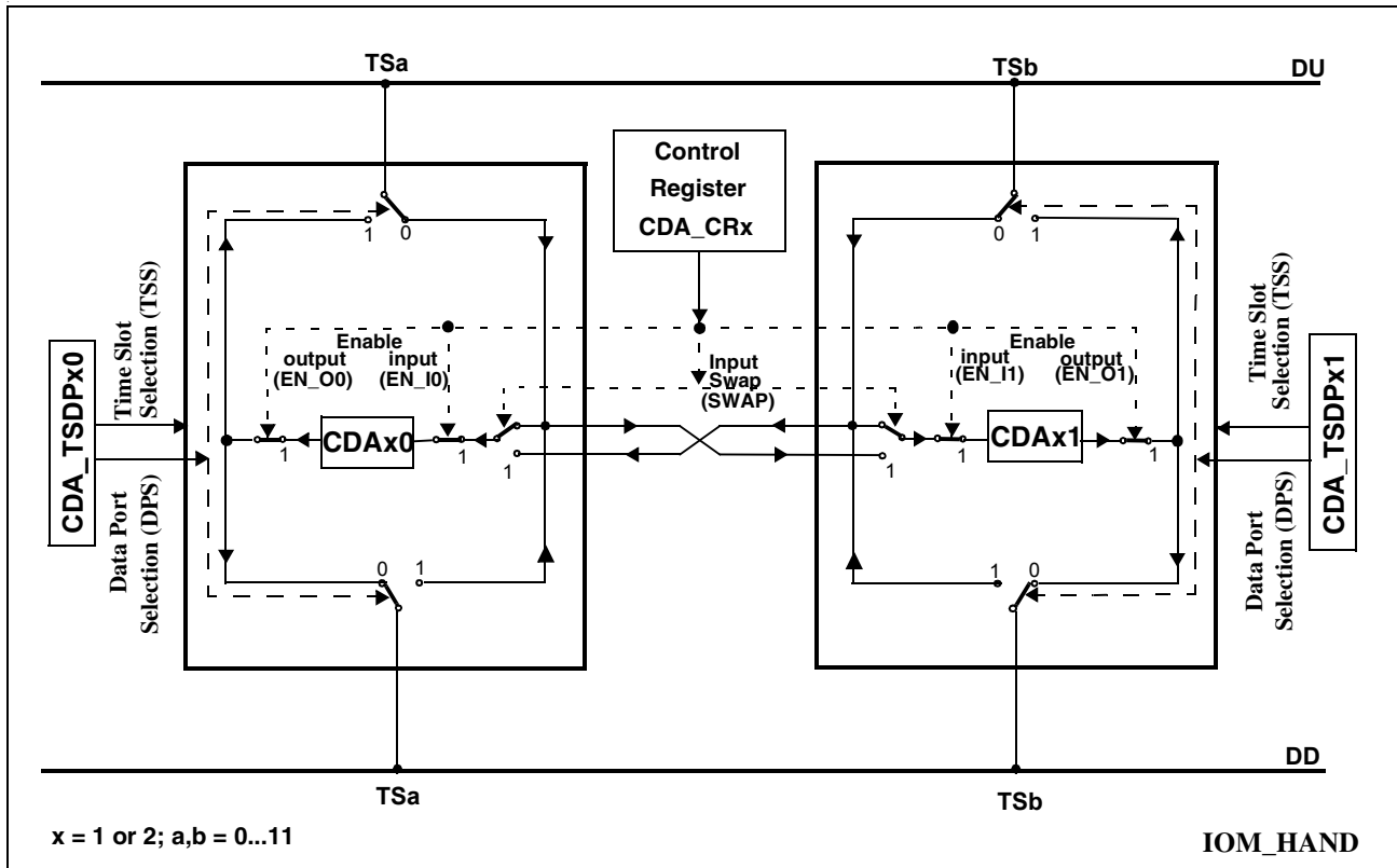
Figure 13 Data Access via CDAX0 and CDAX1 register pairs
