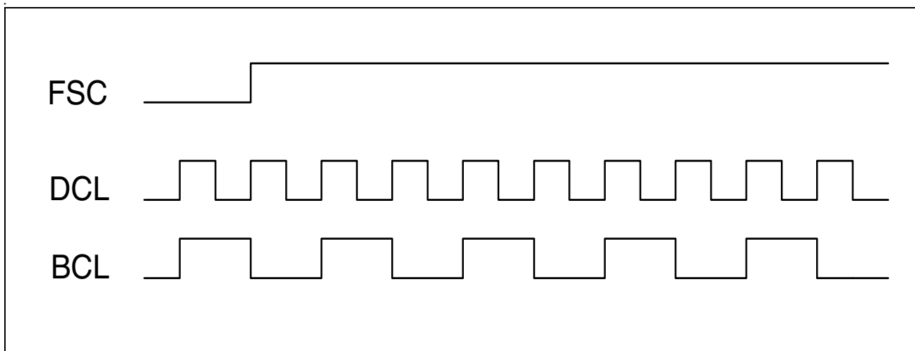
Figure 74 Clock waveforms
