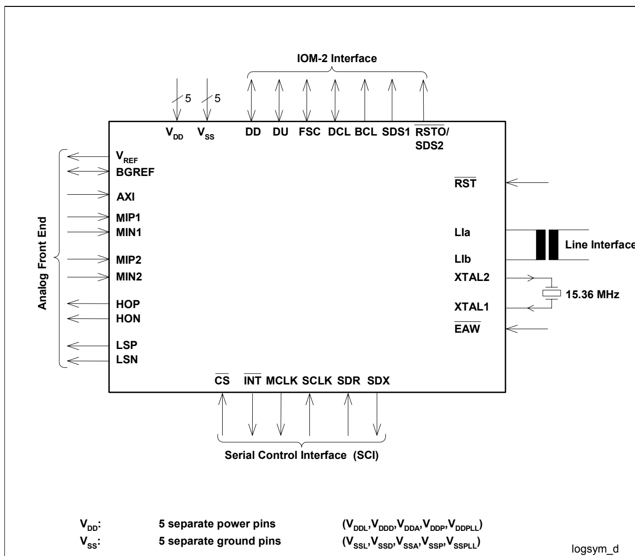
Figure 2 Logic Symbol of the SCOUT-DX in P-MQFP-44
