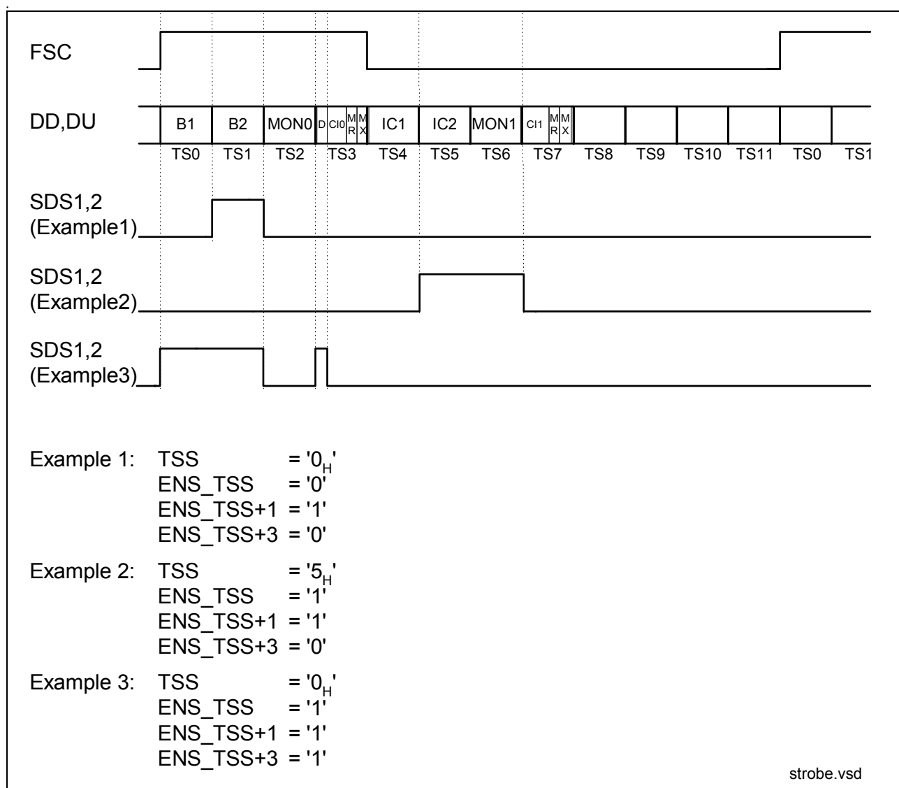
Figure 20 Data Strobe Signal
