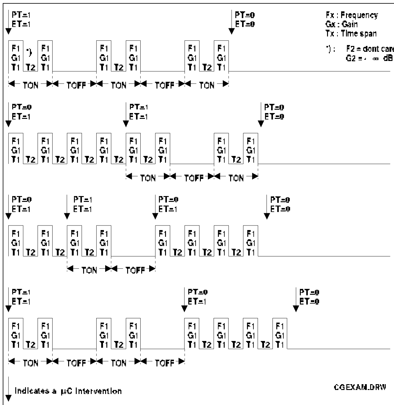
Figure 61 Typical Control Generator Applications
