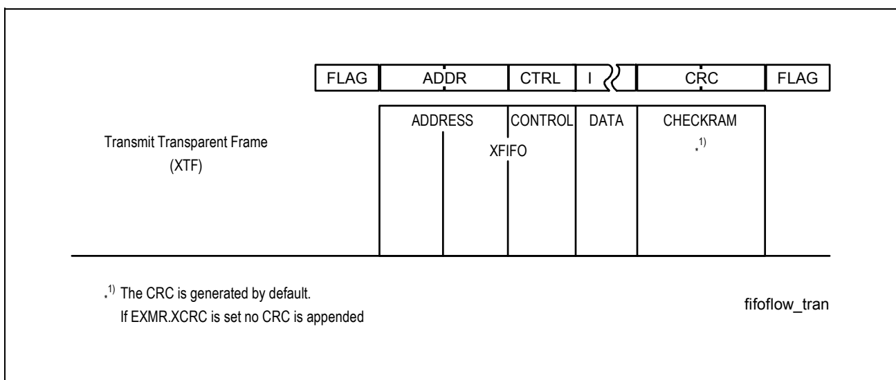
Figure 52 Transmit Data Flow
