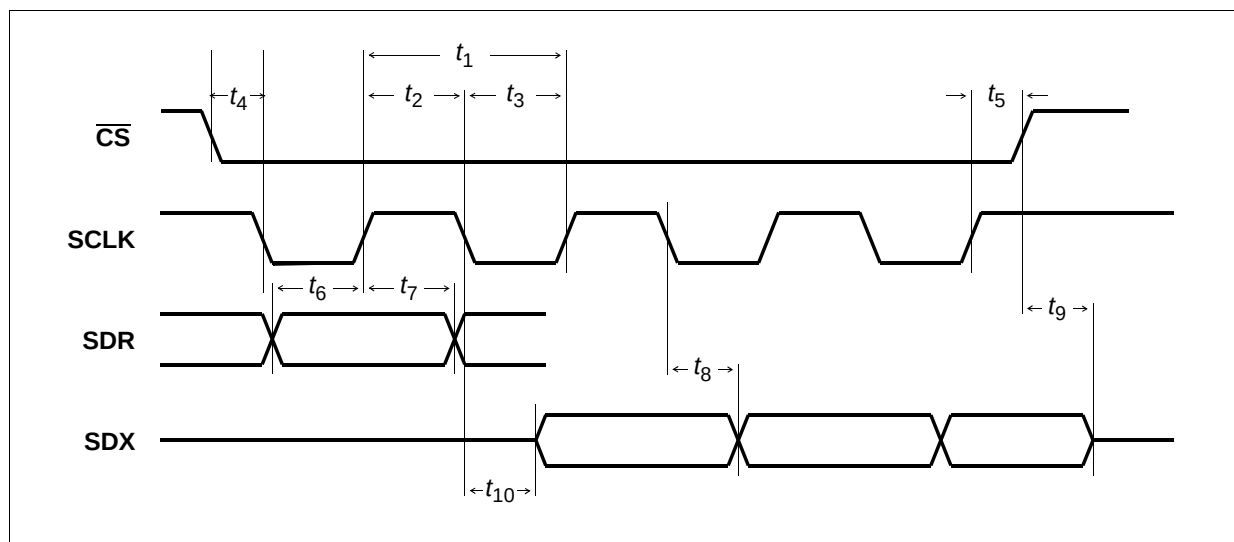
Figure 87 SCI Interface
